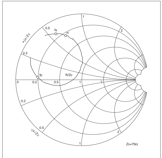
Fig.15 (a) IF Output Impedance of the Tuner
