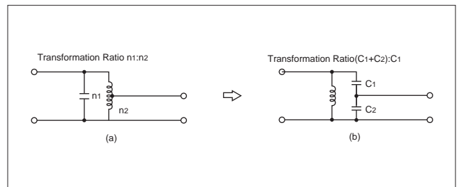
Fig.23 Transformation Circuits
