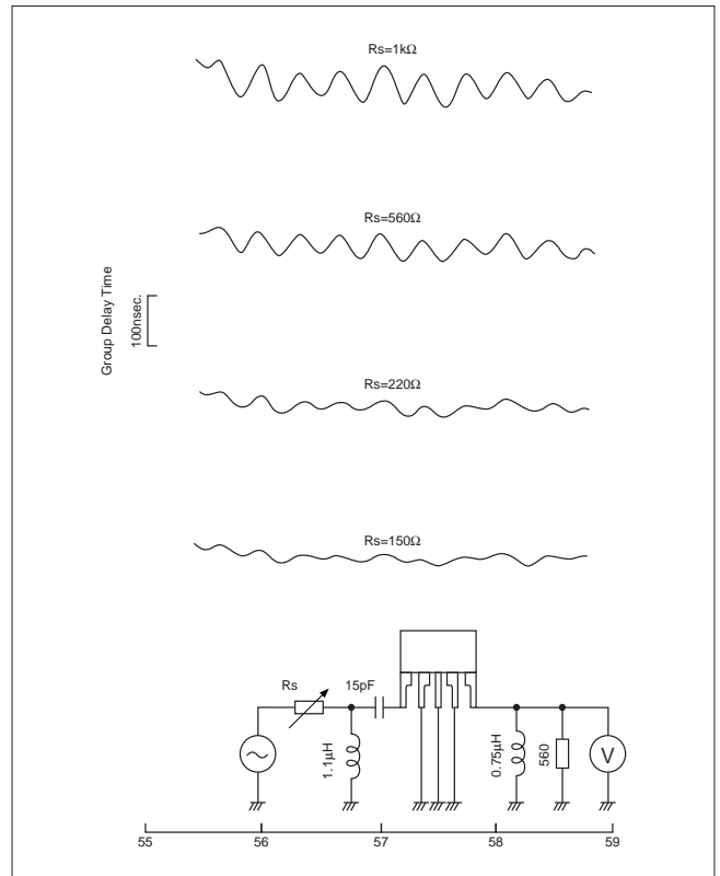
Fig.17 Relation between the Terminating Impedance and the Ripple of the Group Delay Time Characteristic (Parallel tuning)
