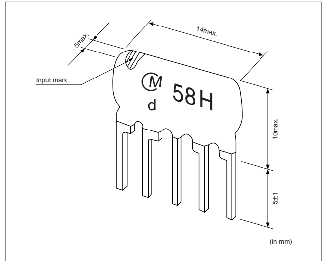
Fig.1 Dimensions
