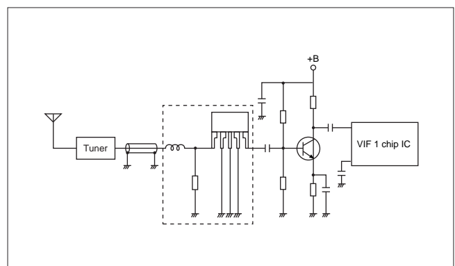
Fig.29 Use of a High Impedance Type SAW Filter in the Postamplifier System
