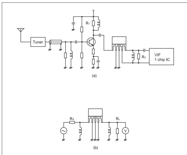
Fig.16 Preamplifier System
