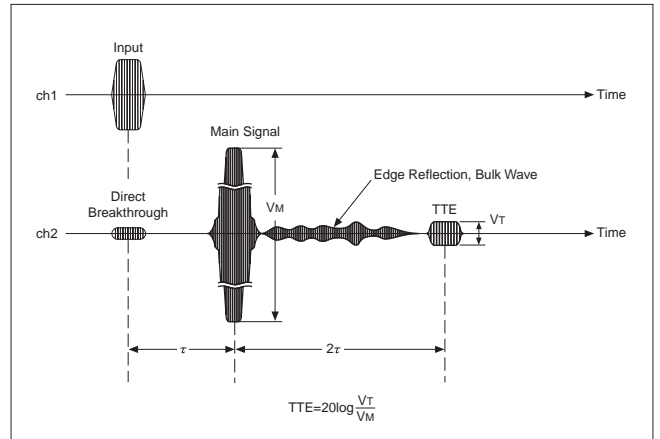
Fig11 Typical Pulse Response Waveform
