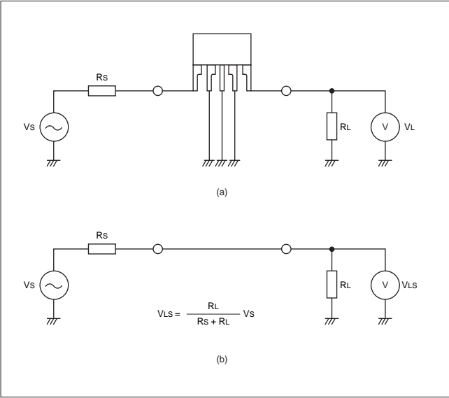
Fig.8 Effect of power dissipation by incorrect insertion of SAW filter
