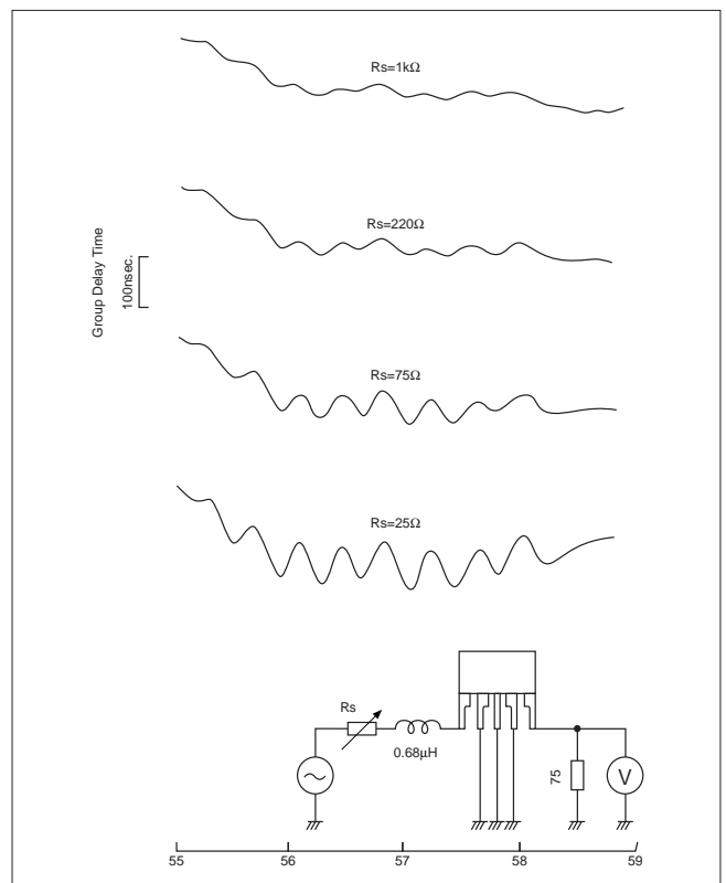
Fig.18 Relation between the Terminating Impedance and the Ripple of the Group Delay Time Characteristic (Series Tuning)
