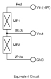
Equivalent Circuit
