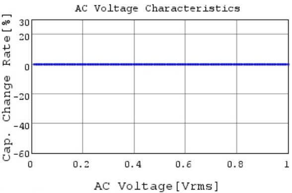
ECASD40E477M006KA0 C-AC Voltage capchange, 1
