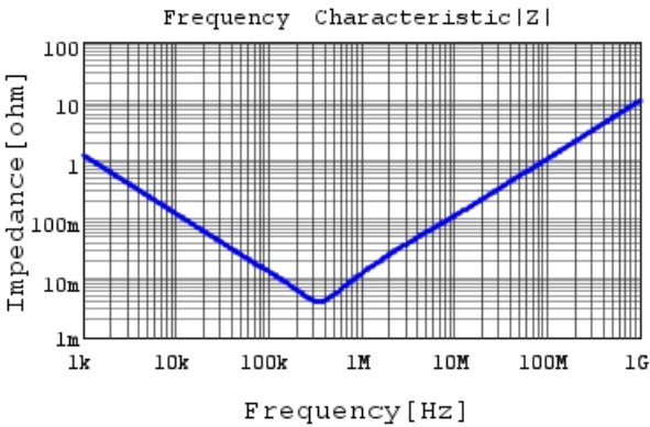
ECASD61A157M010KA0 |Z| DCOV,25degC
