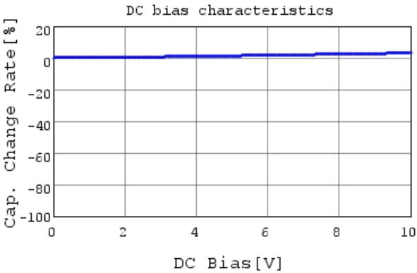
ECASD61A157M010KA0 C-DC bias capchange, 25.0
