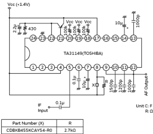
Measurement Circuit
