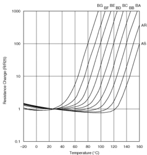
Resistance-Temperature Characteristics
