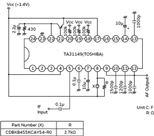
Measurement Circuit
