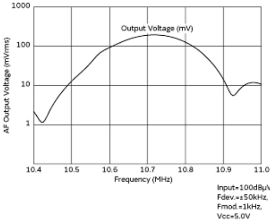
Frequency Characteristics
