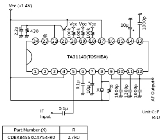
Measurement Circuit
