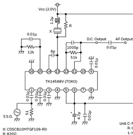
Measurement Circuit
