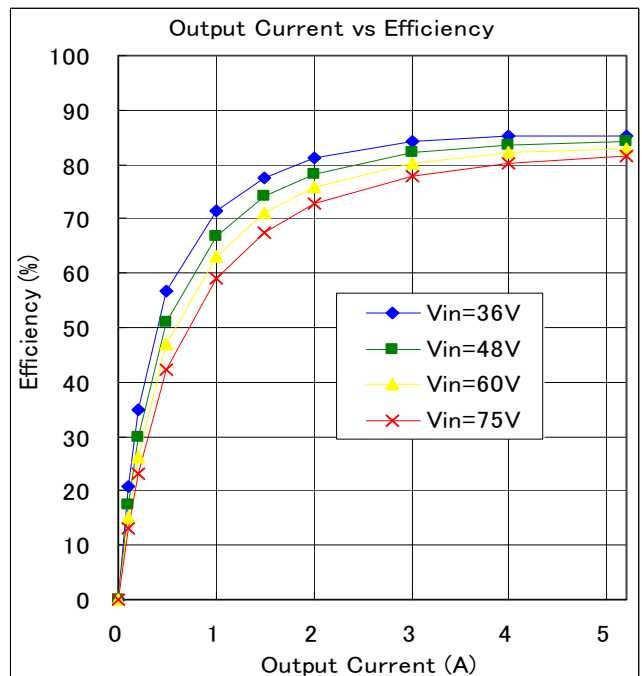
Fig.11-2-2. Efficiency vs Output Current
