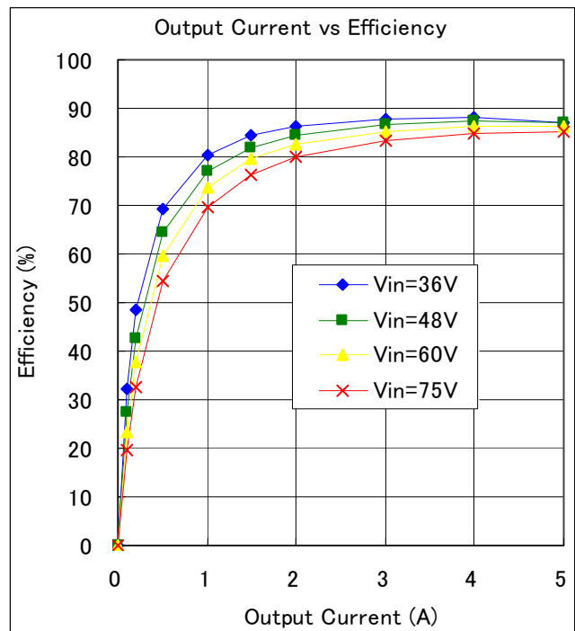
Fig.11-3-2. Efficiency vs Output Current
