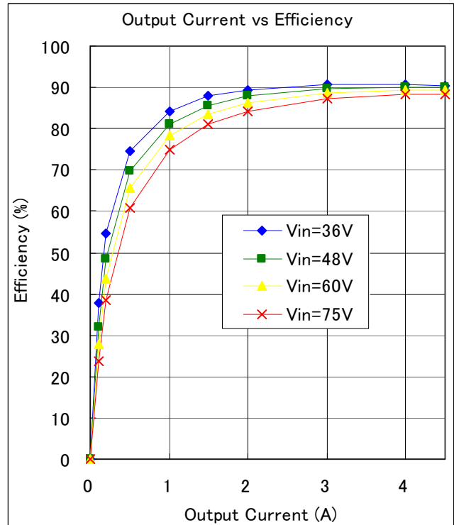
Fig.11-5-2. Efficiency vs Output Current
