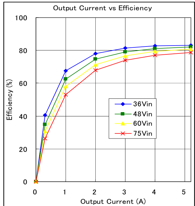
Fig.11-1-2. Efficiency vs Output Current
