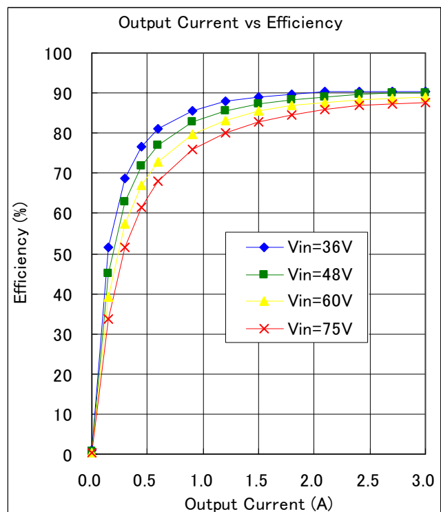
Fig.11-6-2. Efficiency vs Output Current
