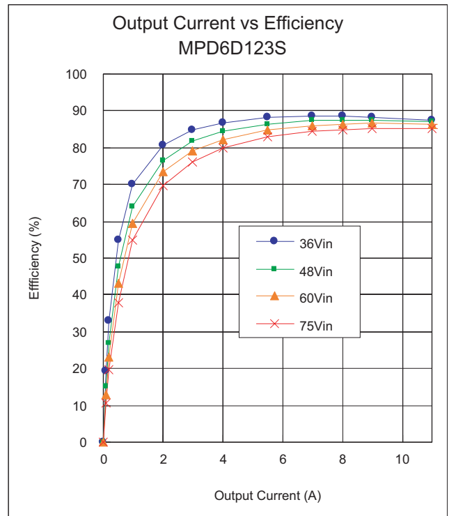
Fig.11-2-2. Efficiency vs Output Current
