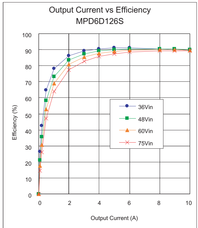
Fig.11-4-2. Efficiency vs Output Current
