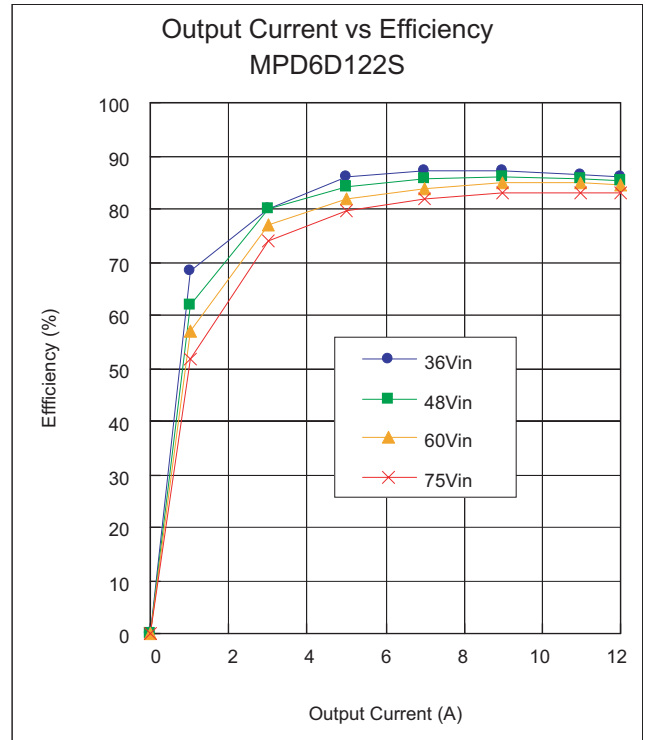
Fig.11-1-2. Efficiency vs Output Current
