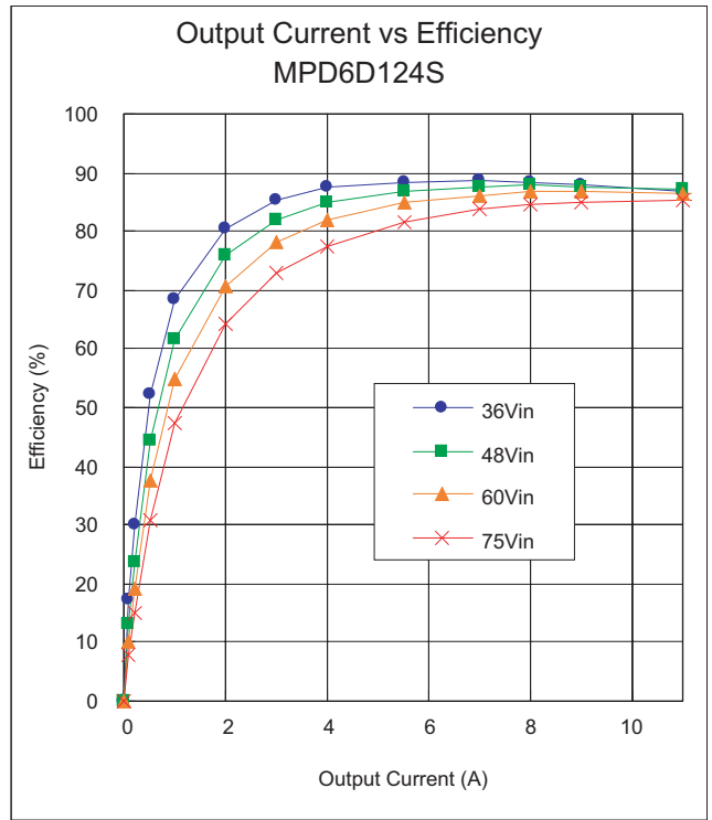
Fig.11-3-2. Efficiency vs Output Current
