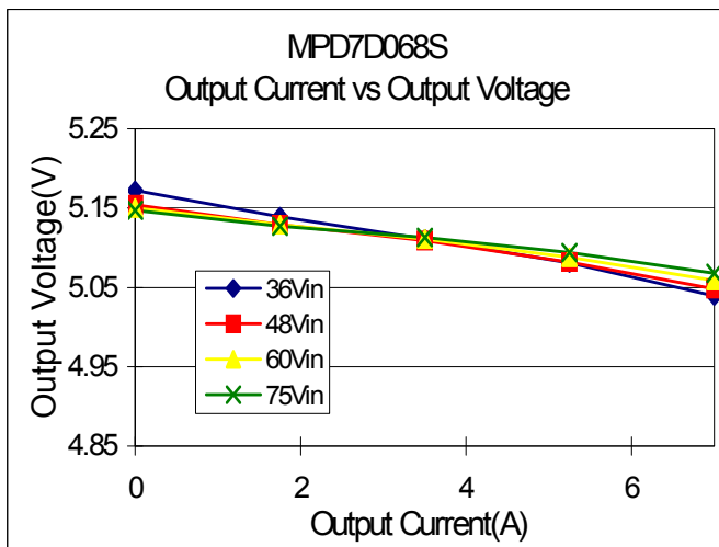
Fig.12-1-1 Output Current vs Output Voltage
