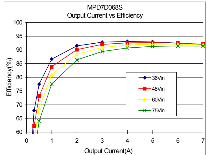
Fig.12-1-2 Output Current vs Efficiency
