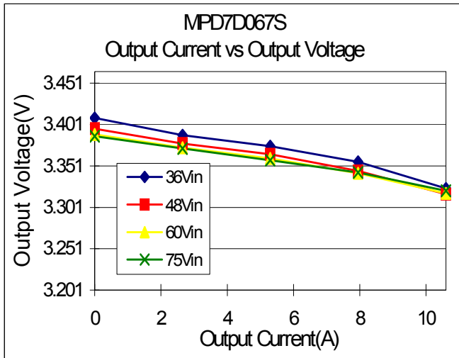
Fig.11-1-1 Output Current vs Output Voltage
