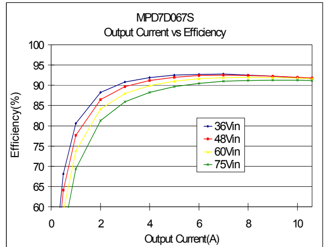
Fig.11-1-2 Output Current vs Efficiency
