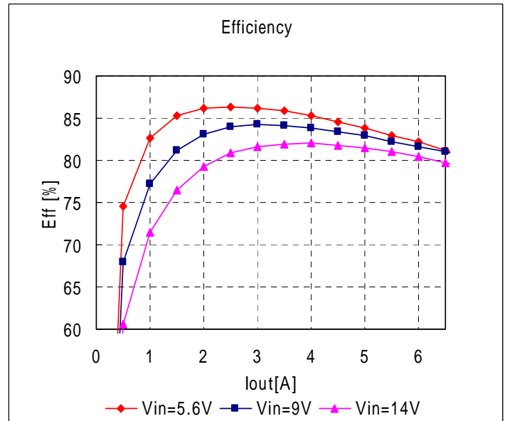
Fig.7-3-14. Efficiency v.s. Output Current
