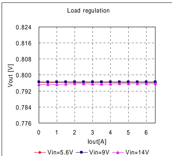
Fig.7-3-16. Output Voltage v.s. Output Current
