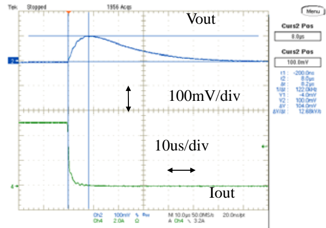
Fig.7-1b. Load Transient Response (MPDRX308S)
