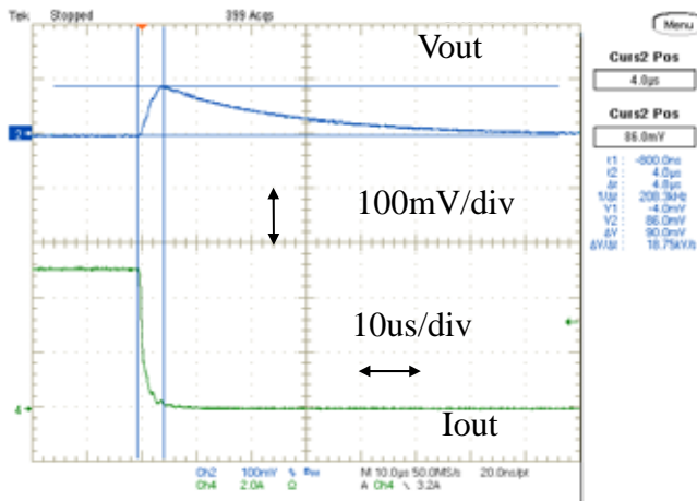
Fig.7-1a. Load Transient Response (MPDRX307S)
