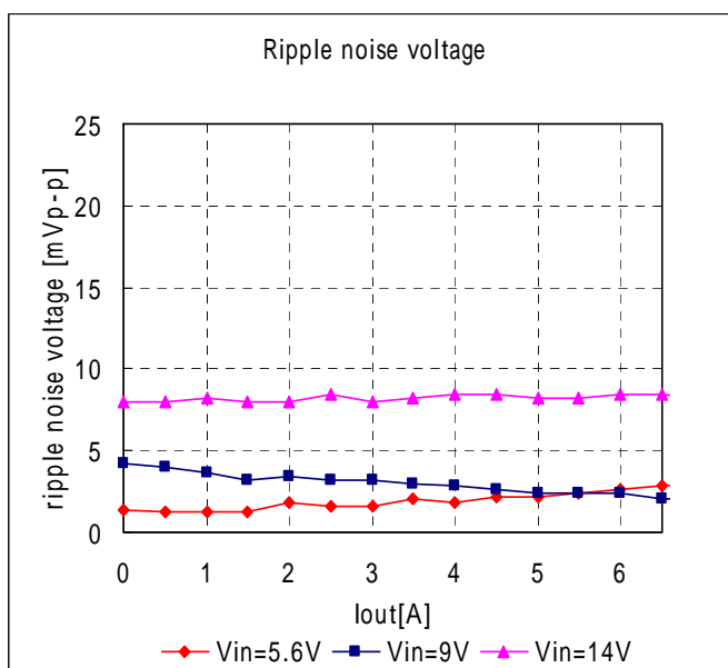
Fig.7-3-18. Ripple Voltage v. s. Output Current
