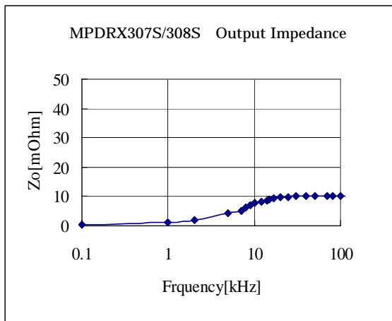
Fig.7-2-1. Output Impedance of MPDRX307S/308S
