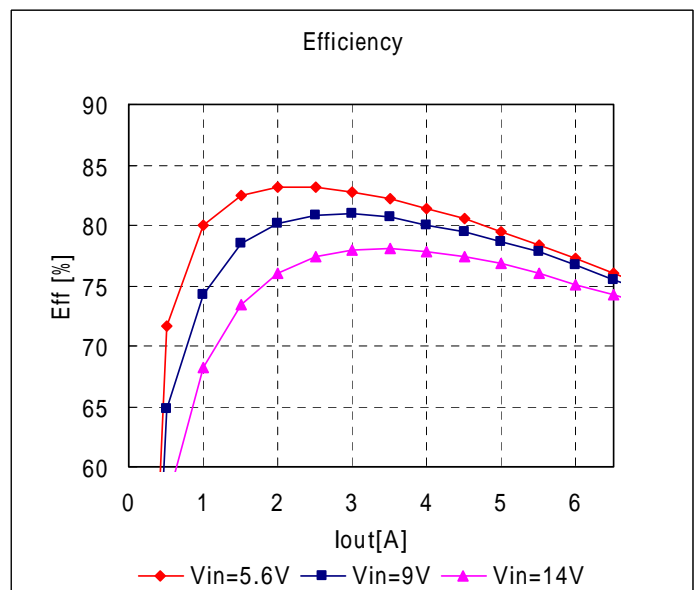
Fig.7-3-17. Efficiency v.s. Output Current
