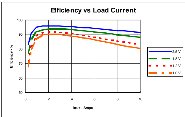
Characteristic Data; Vin =3.3 V (See Note A)
