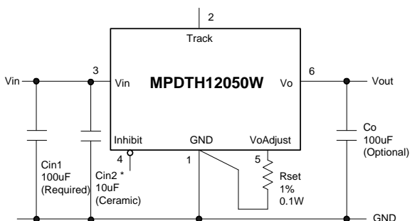
Figure 2-1: Vo Adjust Resistor Placement
