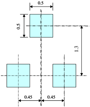
Reference mount pad
