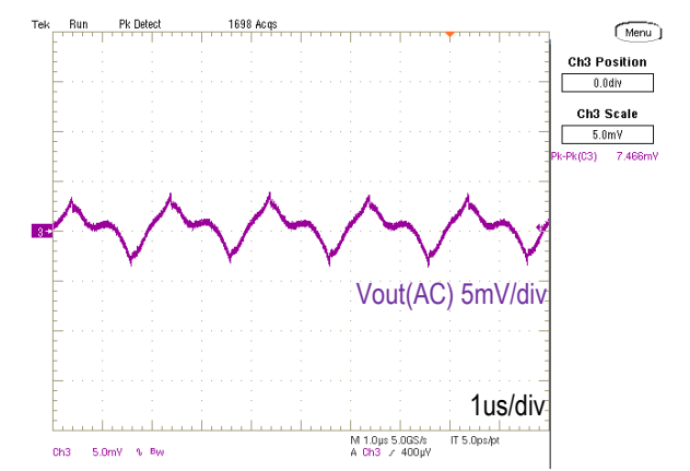
Output Ripple and Noise (Vin=5.0V, Vout=1.8V, Iout=20A, Load=660uF, Scope BW=20MHz, 5mV/div, 1us/div)
