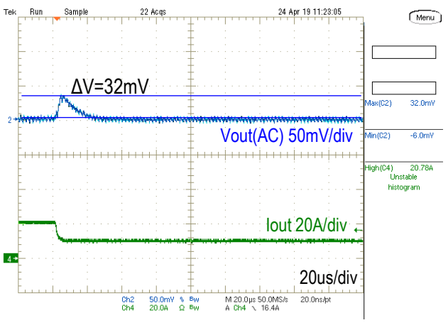
Step Load Transient Response (Vin=5.0V, Vout=1.8V, Load=660uF, Iout=20 to 10A, 1.0A/us) Trace 2=Vout(AC), 50mV/div, Trace 4=Iout, 20A/div, 20us/div
