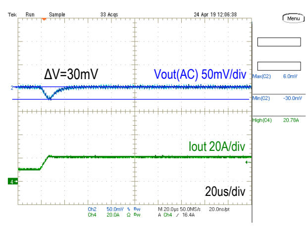
Step Load Transient Response (Vin=5.0V, Vout=0.7V, Cload=660uF, Iout=10A to 20A 1.0A/us) Trace 2=Vout(AC) 50mV/div, Trace 4=Iout 20A/div, 20us/div
