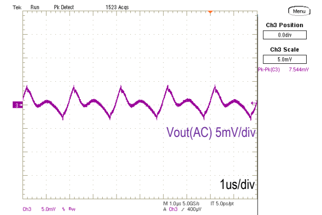
Output Ripple and Noise (Vin=5.0V, Vout=1.0V, Iout=20A, Load=660uF, Scope BW=20MHz, 5mV/div, 1us/div)
