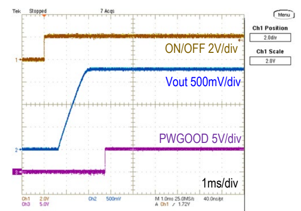
On/Off Enable Delay (Vin=5.0V, Vout=1.8V, Iout=20A, Load=660uF) Trace1=ON/OFF 2V/div, Trace2=Vout 500mV/div, Trace3=PWGOOD 5V/div, 1ms/div
