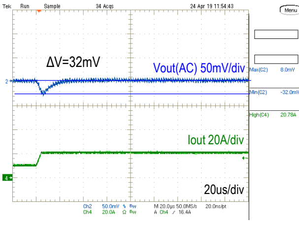
Step Load Transient Response (Vin=5.0V, Vout=1.0V, Load=660uF, Iout=10A to 20A, 1.0A/us) Trace 2=Vout(AC), 50mV/div, Trace 4=Iout, 20A/div, 20us/div
