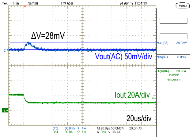
Step Load Transient Response (Vin=5.0V, Vout=1.0V, Load=660uF, Iout=20 to 10A, 1.0A/us) Trace 2=Vout(AC), 50mV/div, Trace 4=Iout, 20A/div, 20us/div
