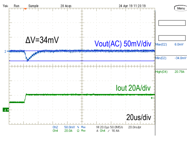
Step Load Transient Response (Vin=5.0V, Vout=1.8V, Load=660uF, Iout=10A to 20A, 1.0A/us) Trace 2=Vout(AC), 50mV/div, Trace 4=Iout, 20A/div, 20us/div
