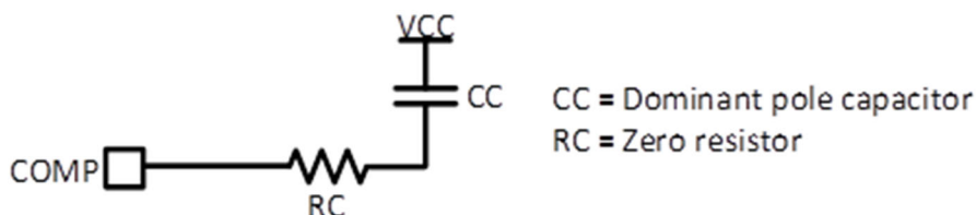
Figure 33. Compensation Components
