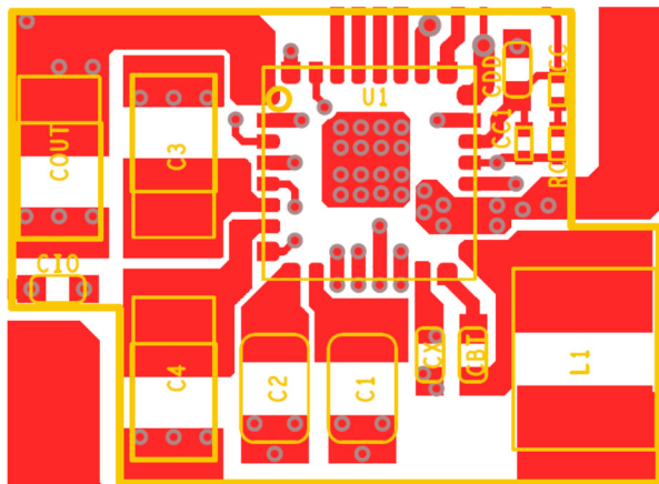
Figure 71: Top Layer
