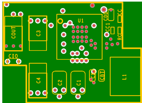
Figure 67: Layer 2
