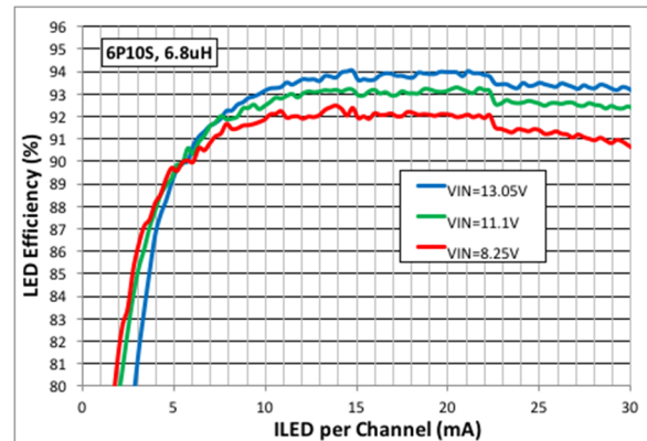
Figure 21: 6P10s LED Efficiency, 6.8 \mu\text{H} Inductor
