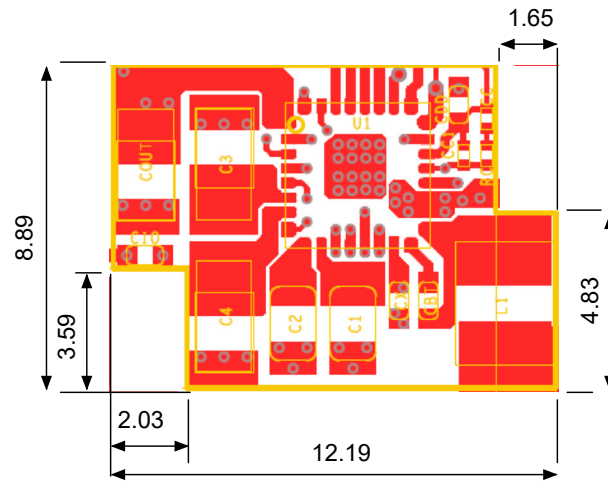
Figure 70: Layout Example
