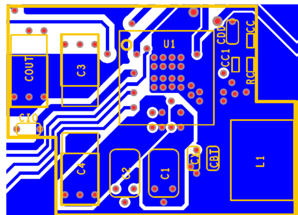
Figure 74: Bottom Layer
