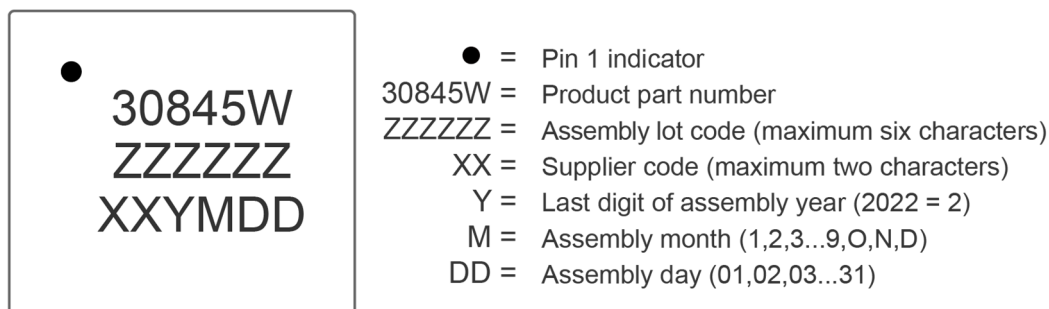
Figure 80: Packaging Marking Information for ARC3C0845W
