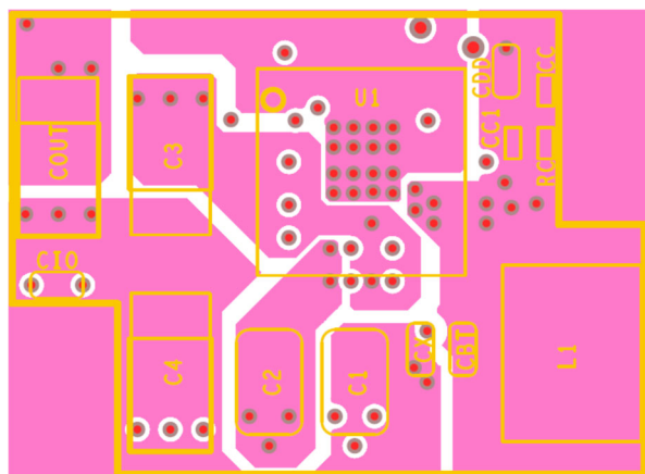
Figure 73: Layer 3
