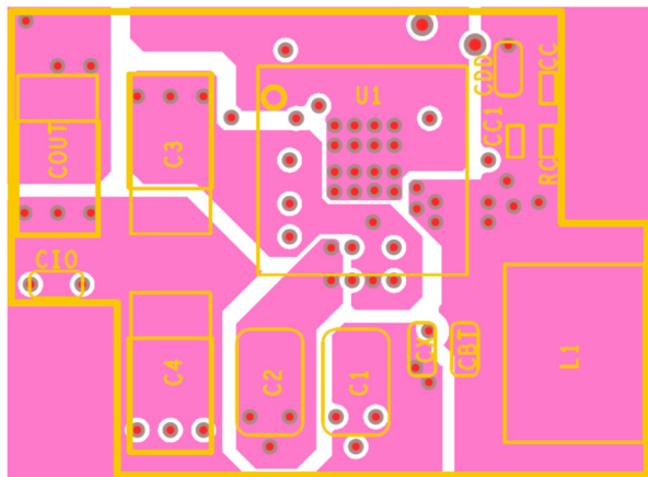
Figure 68: Layer 3
