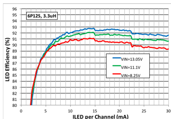
Figure 37: 3S, 6P12s LED Efficiency, 3.3 \mu\text{H} Inductor
