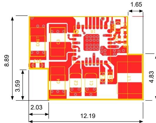
Figure 65: Layout Example
