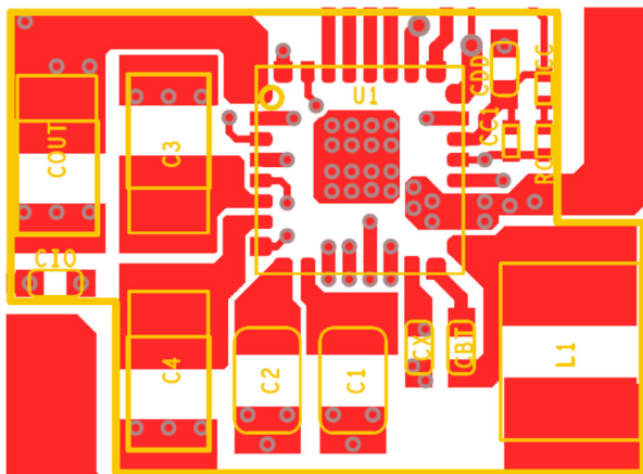
Figure 66: Top Layer
