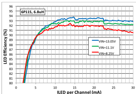
Figure 22: 6P11s LED Efficiency, 6.8 \mu\text{H} Inductor
