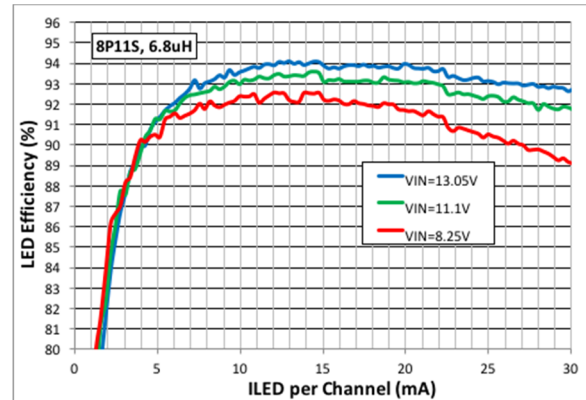
Figure 19: 8P11s LED Efficiency, 6.8 \mu\text{H} Inductor
