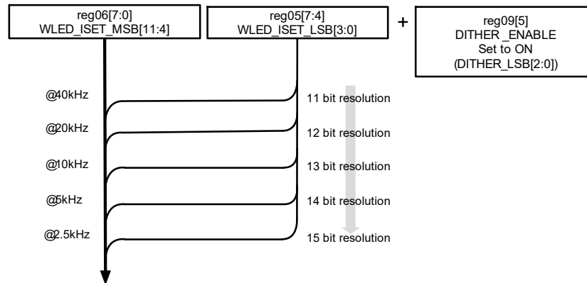
Figure 57: Relationship Between Frequency and Resolution in Phase Shift PWM Dimming with Dither “ON”
