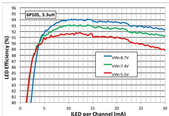
Figure 32: 2S, 6P10s LED Efficiency, 3.3 \mu\text{H} Inductor
