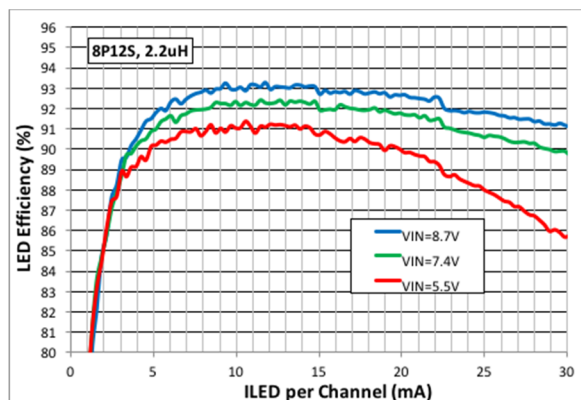
Figure 10: 8P12s LED Efficiency, 2.2 \mu\text{H} Inductor
