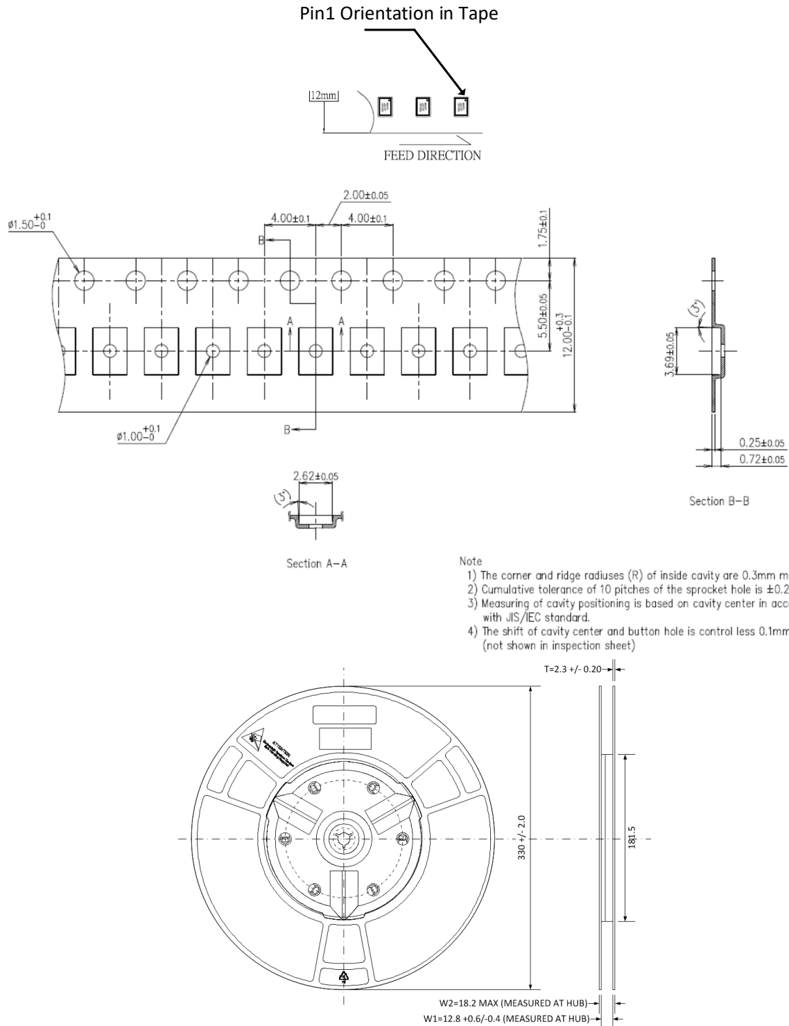
Figure 82: Tape and Reel Information for ARC3C0845W
