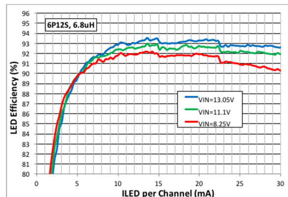
Figure 23: 6P12s LED Efficiency, 6.8 \mu\text{H} Inductor
