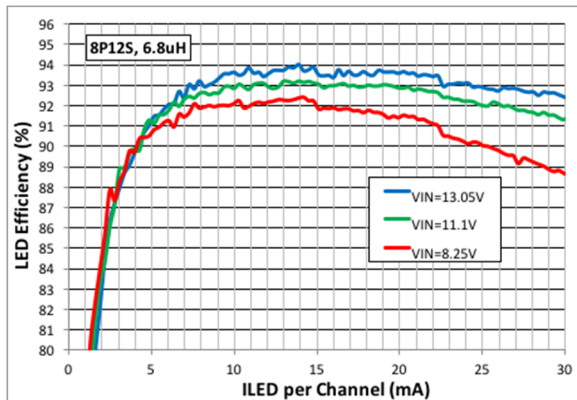
Figure 20: 8P12s LED Efficiency, 6.8 \mu\text{H} Inductor
