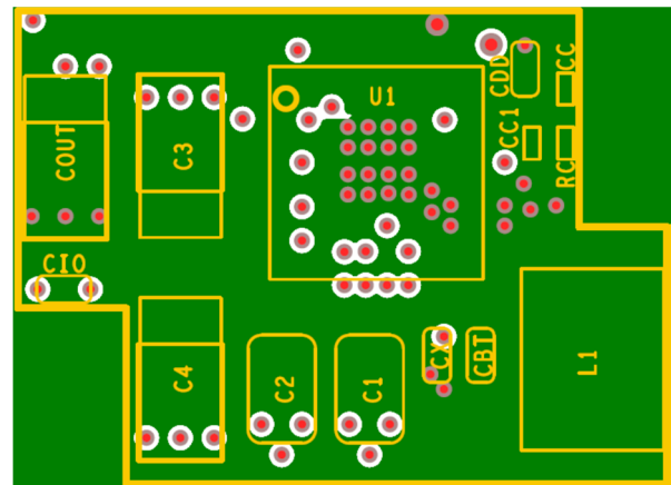
Figure 72: Layer 2
