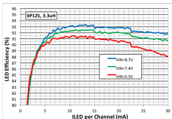
Figure 36: 2S, 6P12s LED Efficiency, 3.3 \mu\text{H} Inductor
