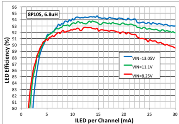
Figure 18: 8P10s LED Efficiency, 6.8 \mu\text{H} Inductor
