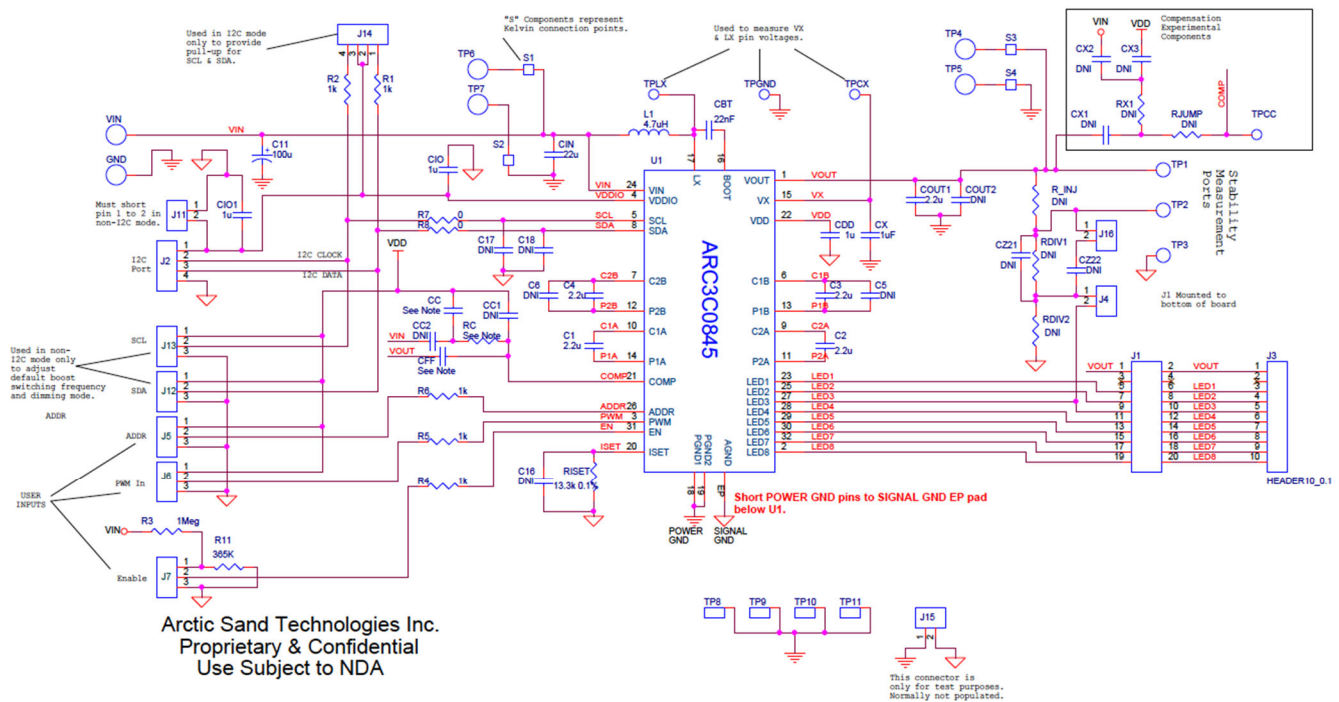
Figure 64: Detailed Application Schematic
