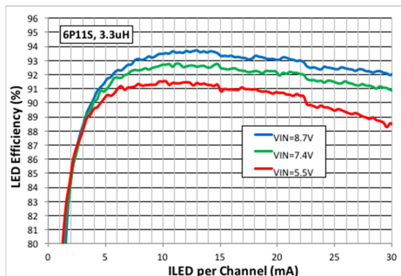
Figure 34: 2S, 6P11s LED Efficiency, 3.3 \mu\text{H} Inductor
