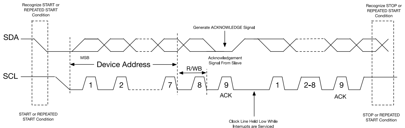
Figure 61: Bus Protocol
