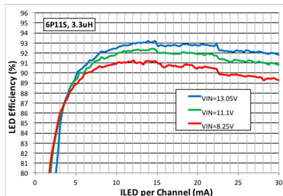
Figure 35: 3S, 6P11s LED Efficiency, 3.3 \mu\text{H} Inductor
