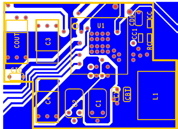
Figure 69: Bottom Layer
