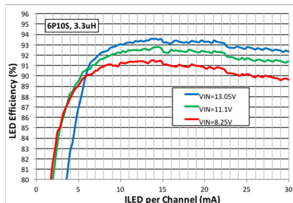
Figure 33: 3S, 6P10s LED Efficiency, 3.3 \mu\text{H} Inductor
