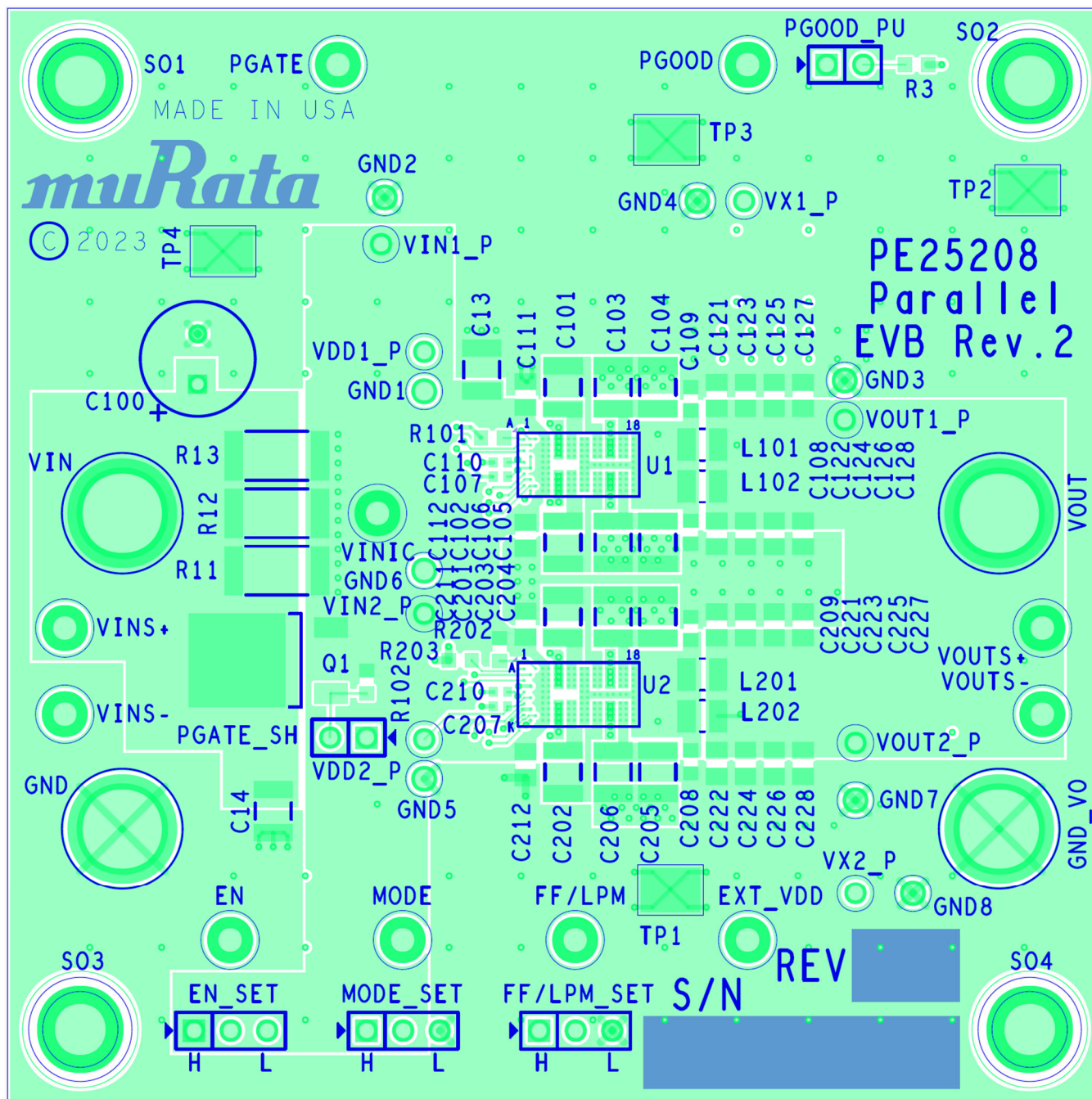
Figure 12. Top Layer (PWR and IC Signal Fanout) PCB Layout of the PE25208 Parallel EVK
