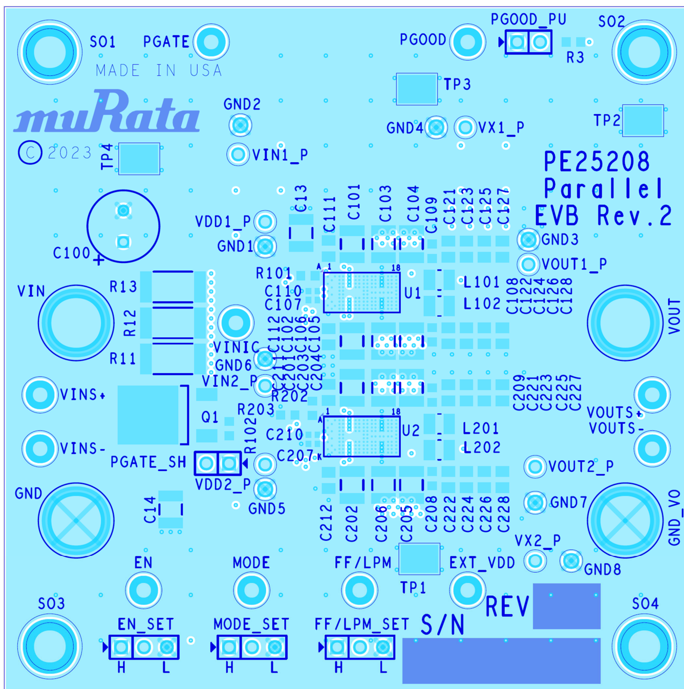
Figure 13. Inner Layer 1 (GND) PCB Layout of the PE25208 Parallel EVK
