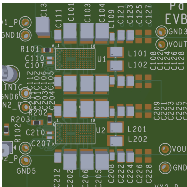
Figure 18. 3D PCB Layout and Critical Component Placement for the Two Parallel PE25208 Devices
