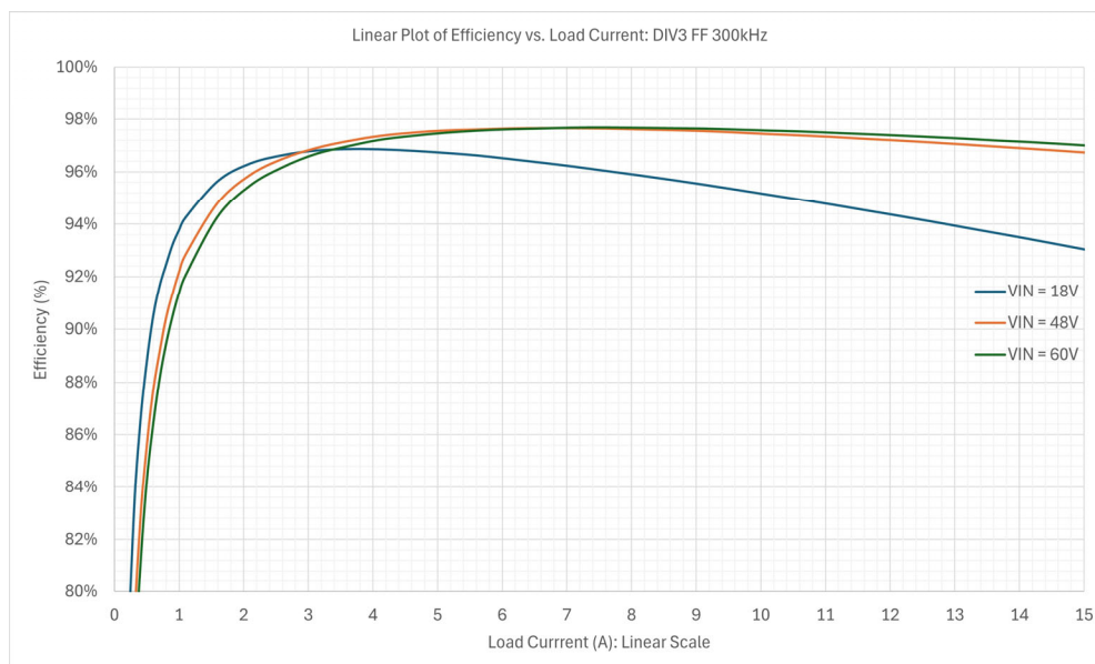
Figure 10. Linear Efficiency (%) vs. Load Current (A) Plot: VIN = (18V, 48V, 60V), DIV3, FF, 300 kHz
