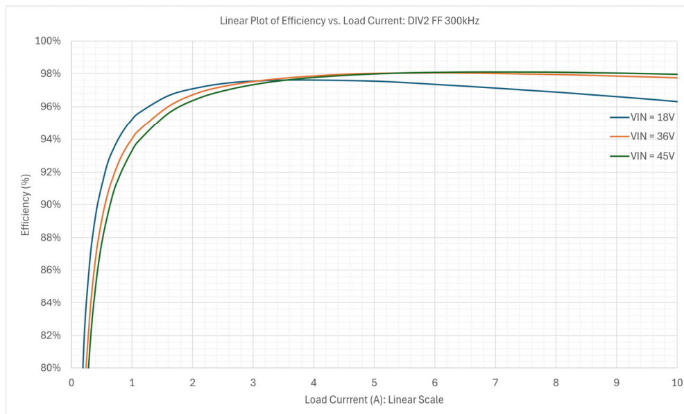
Figure 9. Linear Efficiency (%) vs. Load Current (A) Plot: VIN = (18V, 36V, 45V), DIV2, FF, 300 kHz
