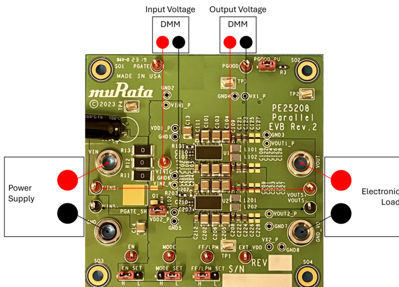
Figure 6. PE25208 Parallel EVK Connections to Equipment for Voltage-only Measurements
