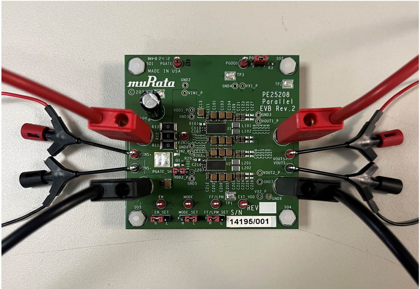
Figure 5. PE25208 Parallel EVK Connection to the Power and Sense Leads
