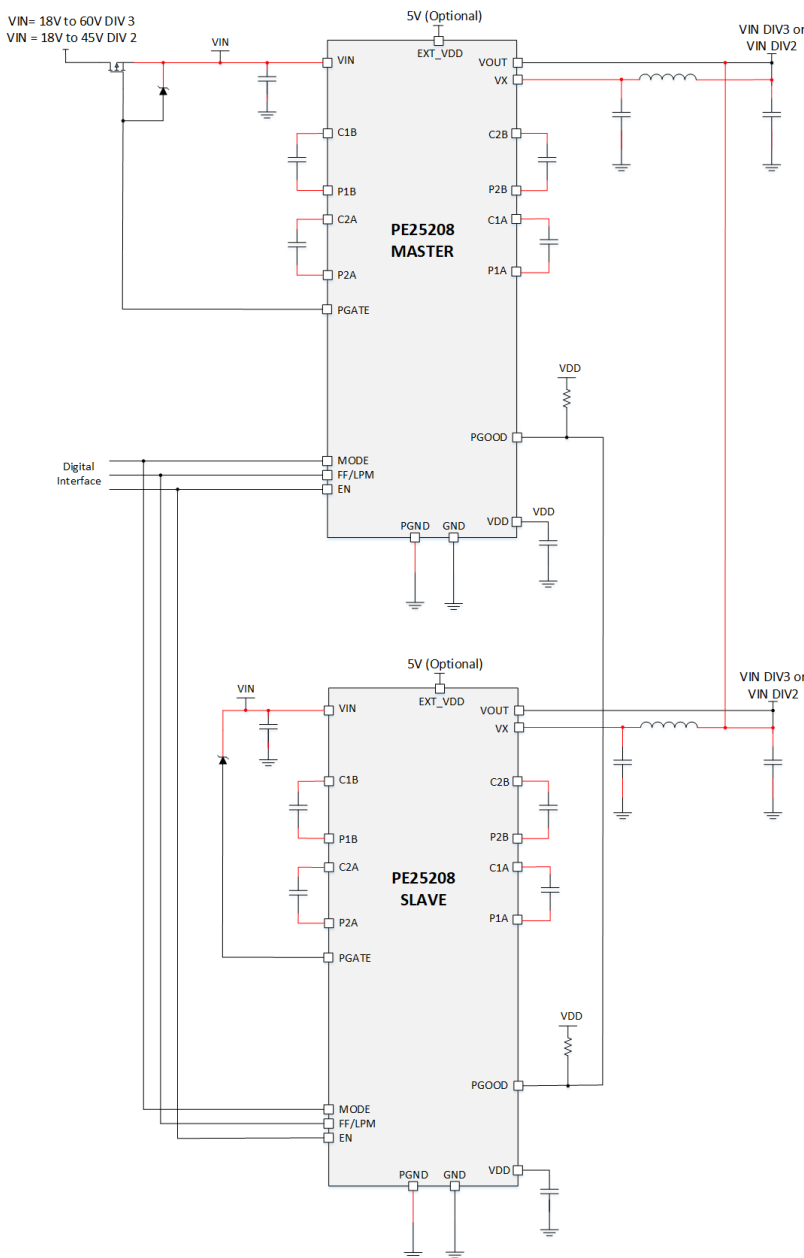
Figure 16. Application Circuit of Two PE25208 Devices in Parallel Operation
