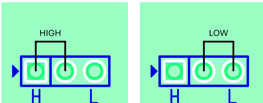
Figure 3. Valid Jumper Configurations for Operation
