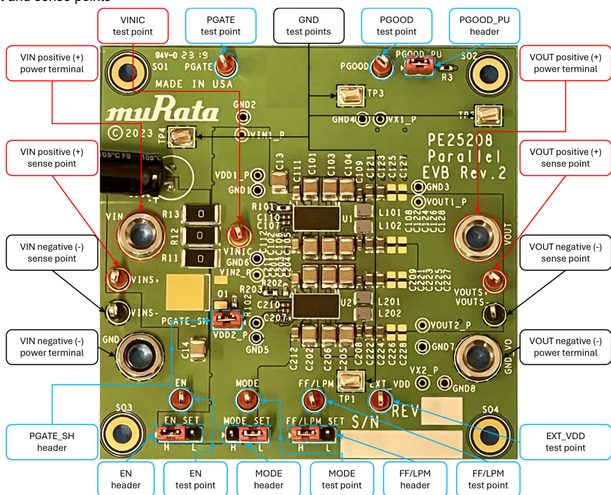
Figure 2. PE25208 Parallel EVK Hardware Interfaces
