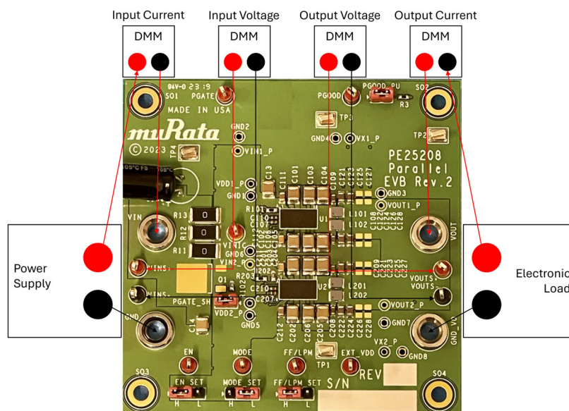
Figure 7. PE25208 Parallel EVK Connections to Equipment for Voltage and Current Measurements
