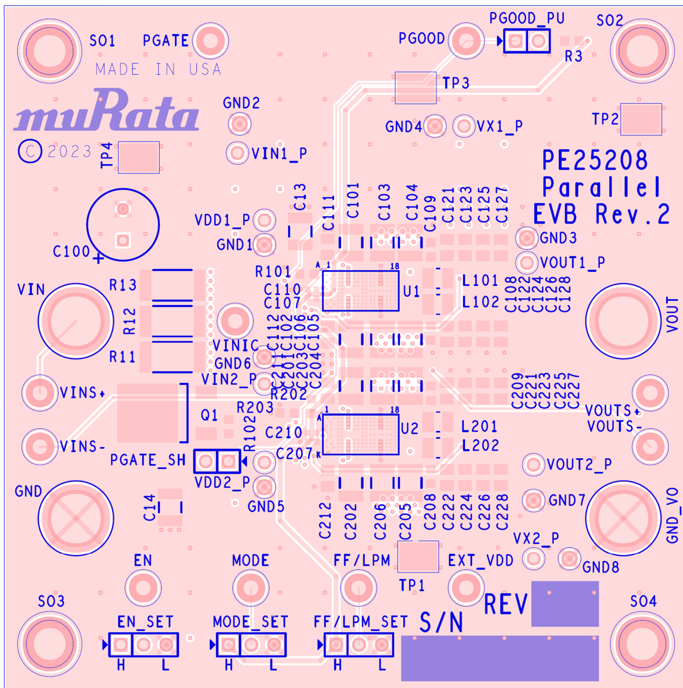
Figure 15. Bottom Layer (Signal) PCB Layout of the PE25208 Parallel EVK
