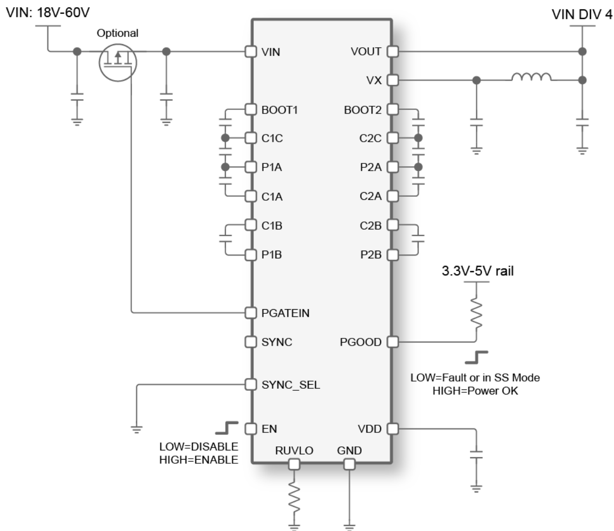
Figure 3. Simplified Application Circuit
