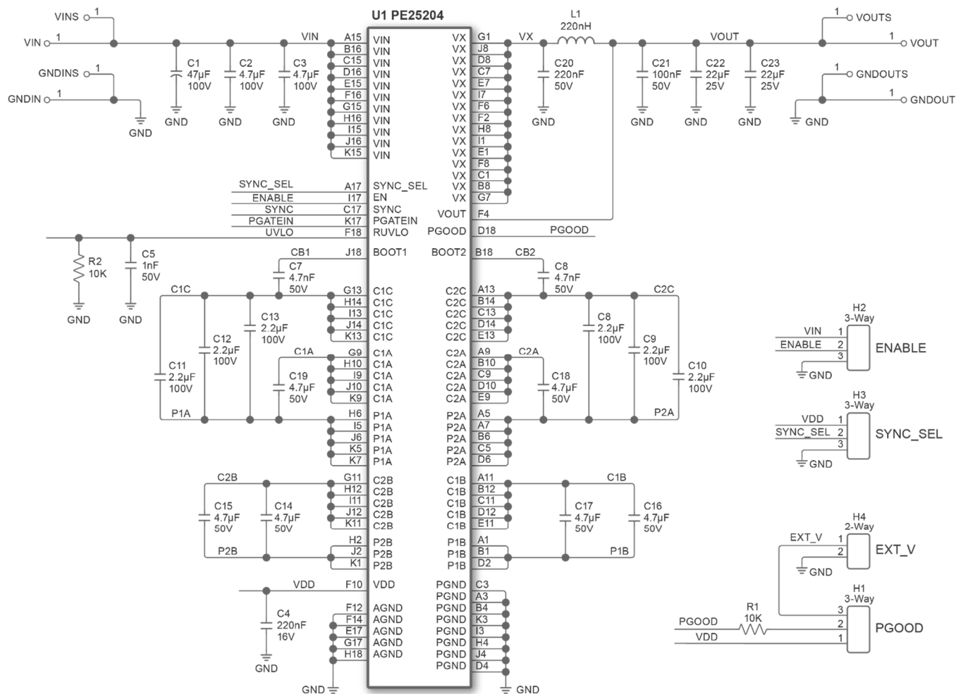
Figure 5. Application Schematic
