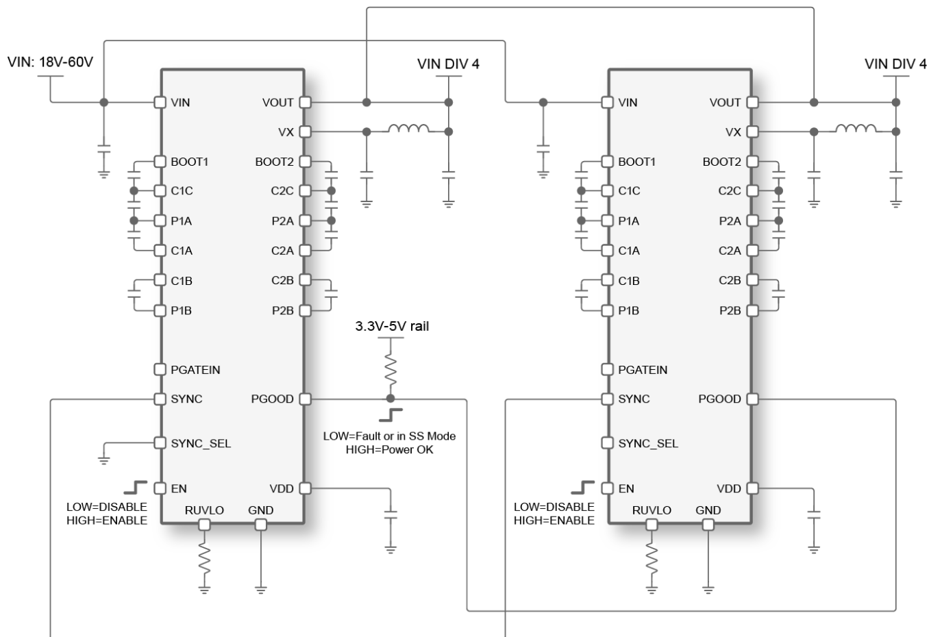
Figure 4. PE25204 Application Circuit in Parallel ICs Operation
