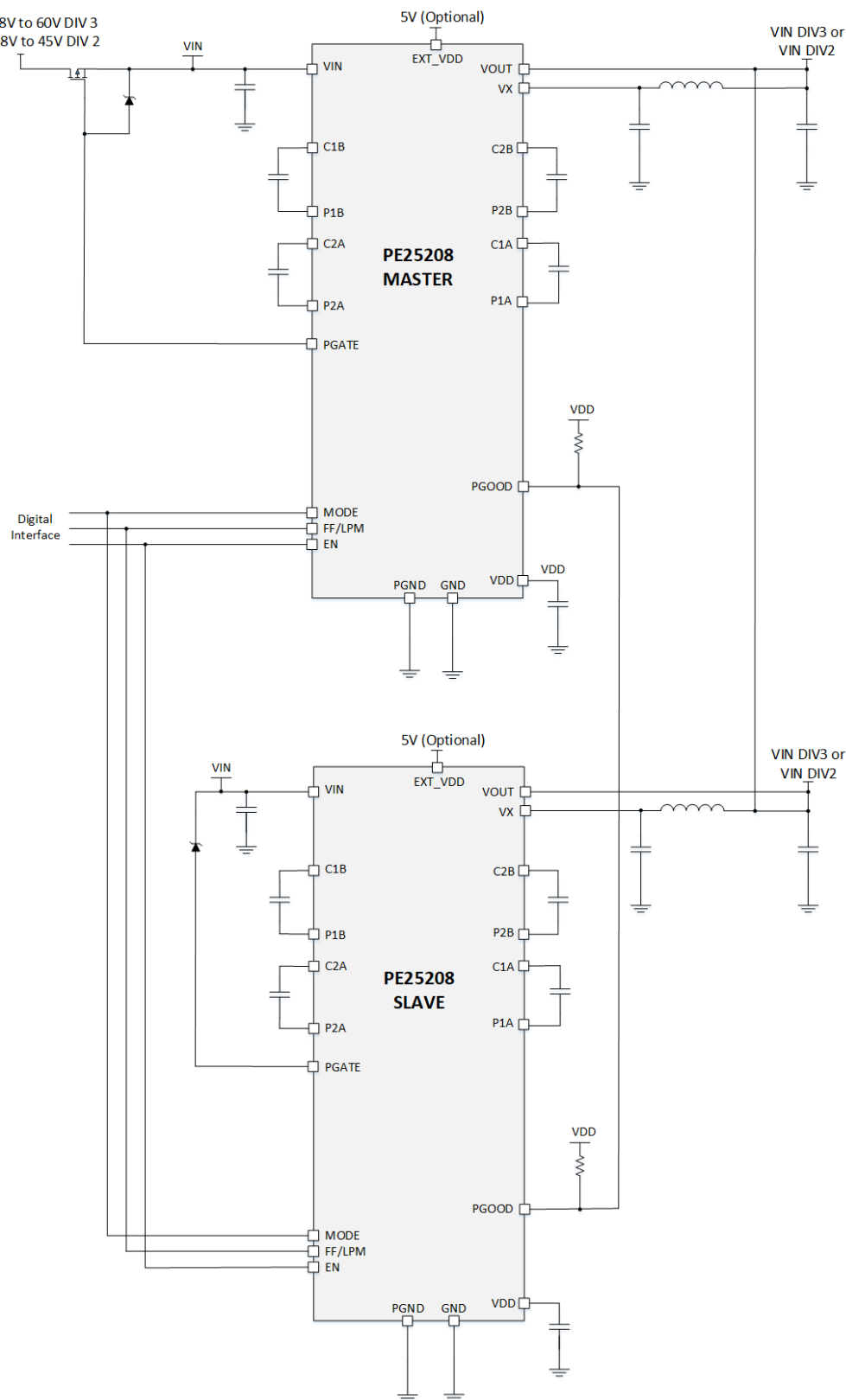
Figure 4. PE25208 Application Circuit in Parallel-IC Operation
