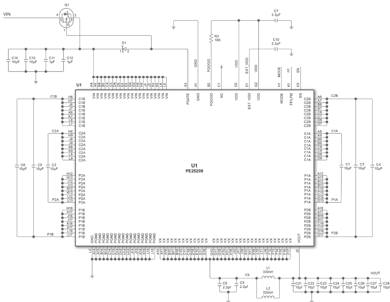
Figure 5. PE25208 Single Application Schematic
