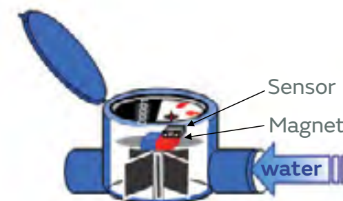
Water meter
