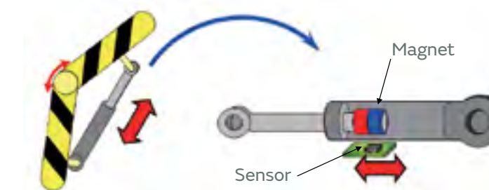
Cylinder control
