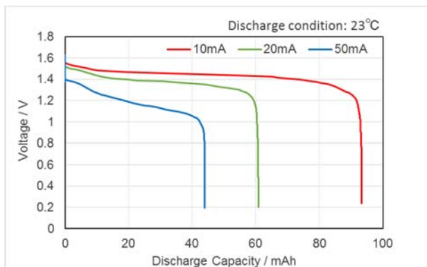
Discharge Characteristics on Load
