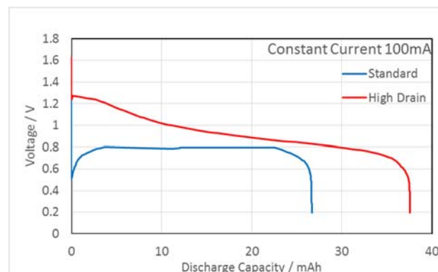
Standard Model vs. High Drain Model
