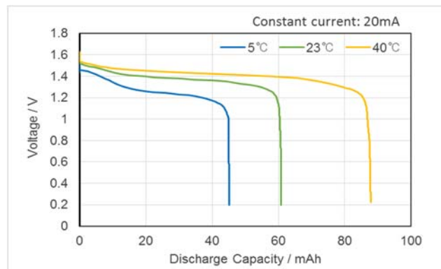
Discharge Characteristics on Temperature
