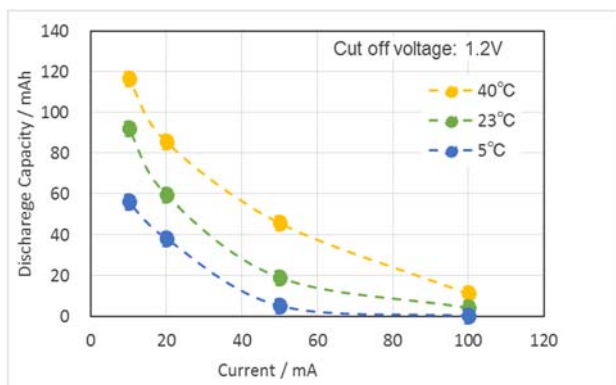
Discharge Load vs. Discharge Capacity
