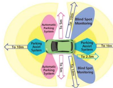
ADAS Applications for Ultrasonic Sensors
