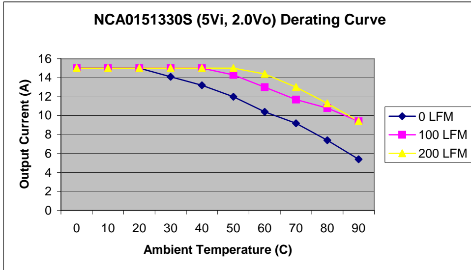
Fig 6. SMT Power Derating vs Output Current for 5V in 2.0V o Out.
