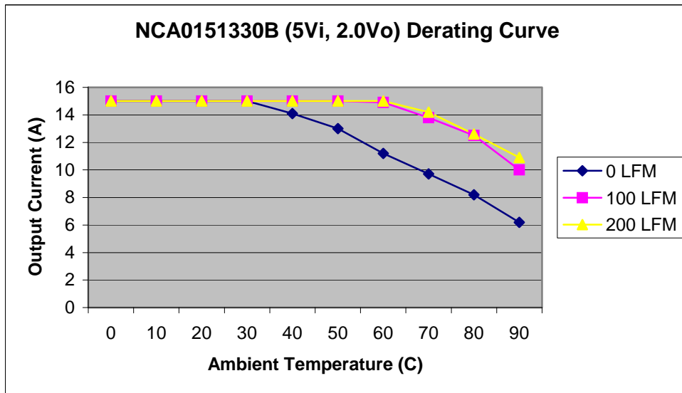
Fig 7. SIP Power Derating vs Output Current for 5V in 2.0V o Out.
