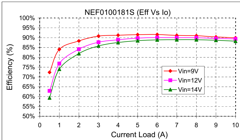
Figure 13. Efficiency Curves for Vout=1.8V (25C)
