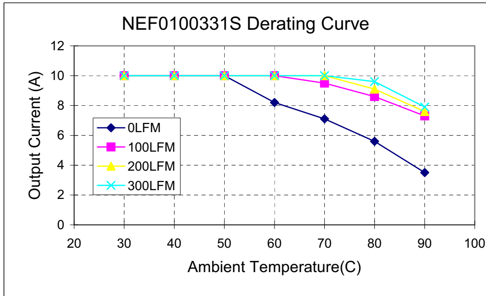
Figure 8. Typical Power Derating vs Output Current for 12Vi and 3.3Vo
