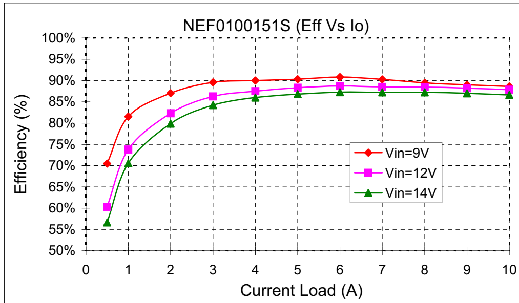
Figure 12. Efficiency Curves for Vout=1.5V (25C)
