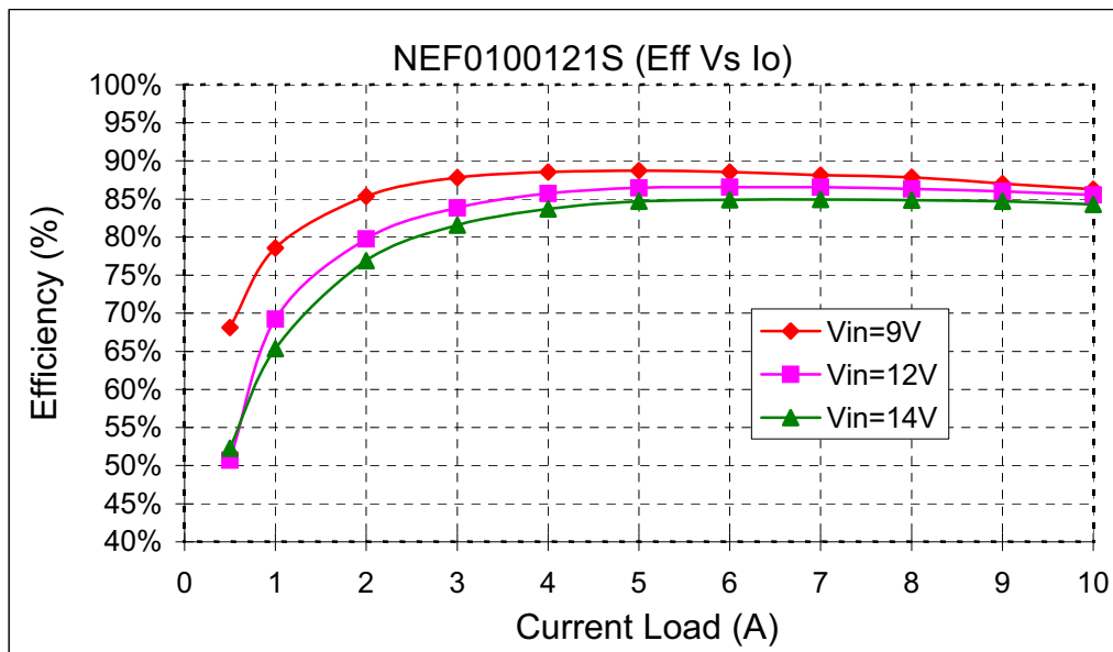
Figure 11. Efficiency Curves for Vout=1.2V (25C)
