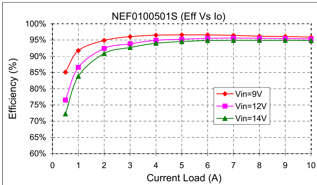
Figure 17. Efficiency Curves for Vout=5.0V (25C)
