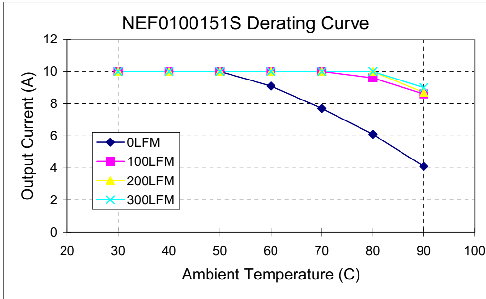
Figure 4. Typical Power Derating vs Output Current for 12Vi and 1.5Vo.
