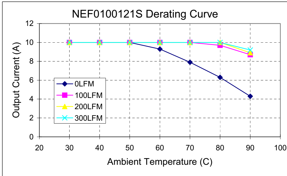
Figure 3. Typical Power Derating vs Output Current for 12Vi and 1.2Vo
