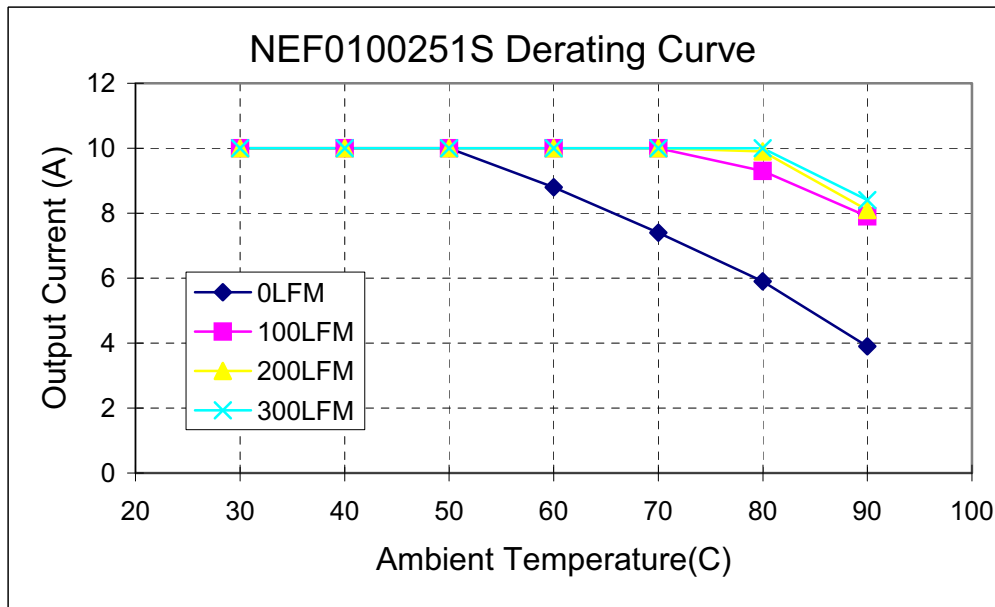
Figure 7. Typical Power Derating vs Output Current for 12Vi and 2.5Vo.
