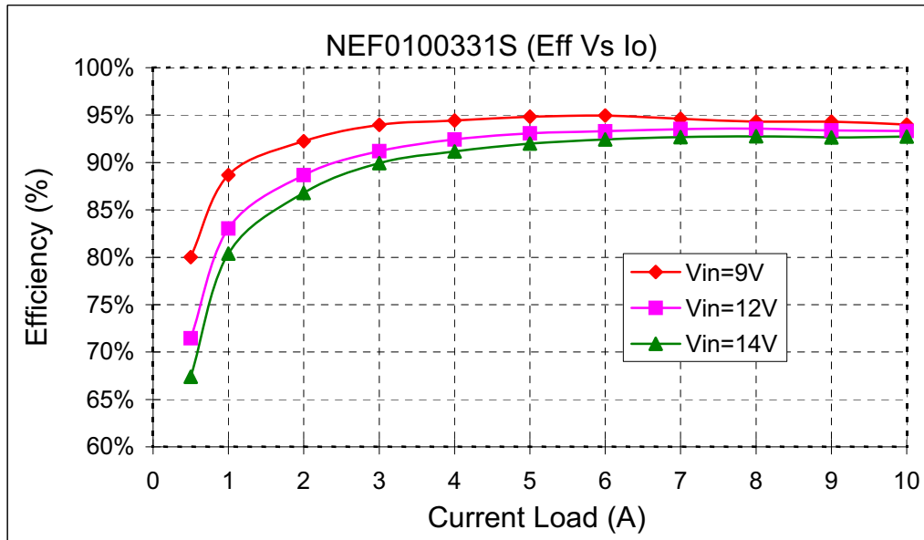
Figure 16. Efficiency Curves for Vout=3.3V (25C)
