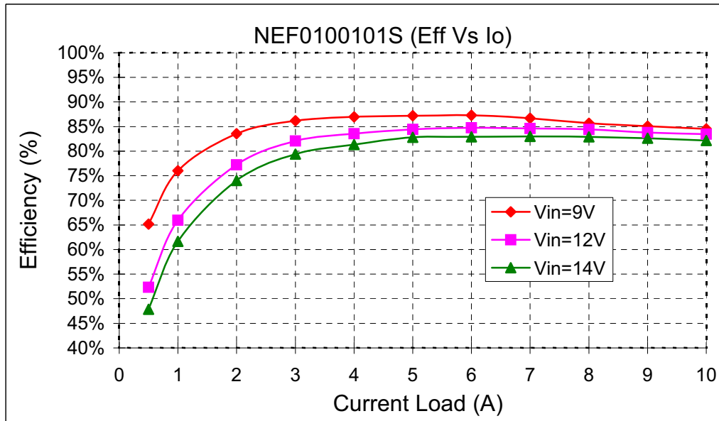
Figure 10. Efficiency Curves for Vout=1.0V (25C)
