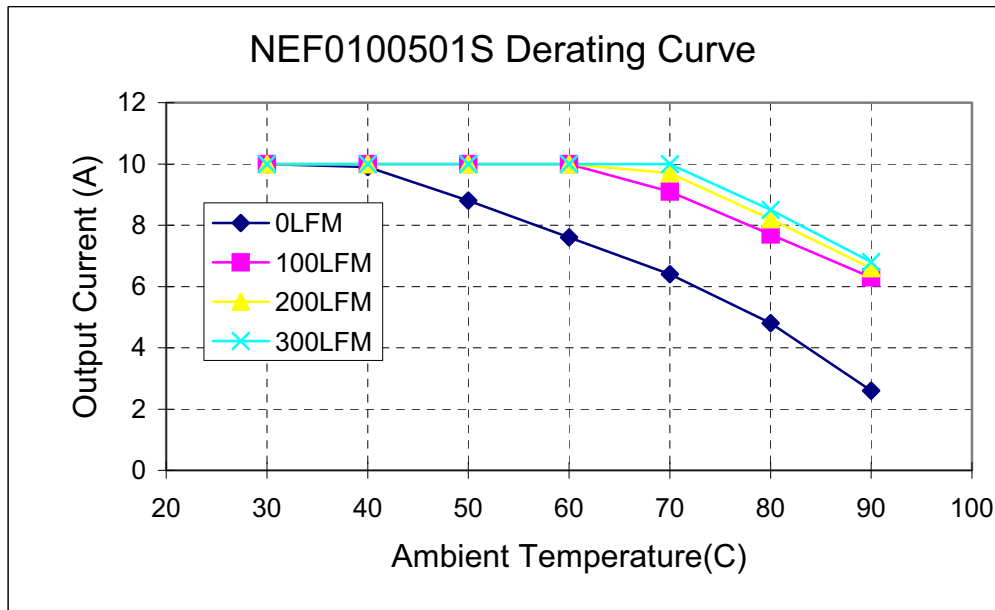
Figure 9. Typical Power Derating vs Output Current for 12Vi and 5.0Vo
