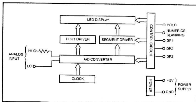
Figure 1. DM-500 Simplified Block Diagram
