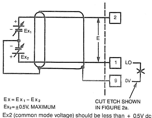
Figure 2b. Typical Differential Input Configuration
