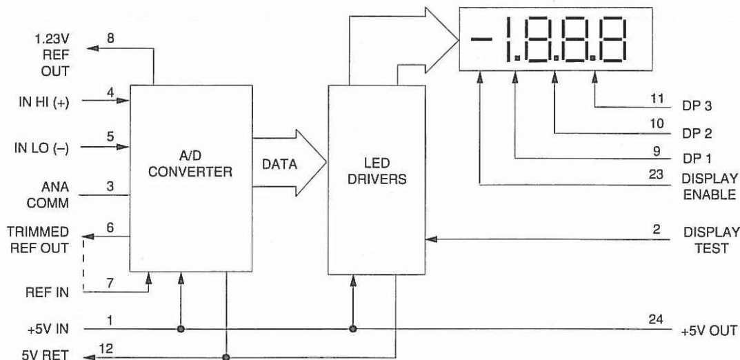
Figure 1. DMH-30 Simplified Block Diagram
