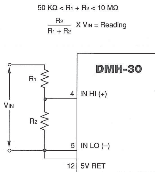
Figure 2. Simple Attenuation Circuit for Scaling Input Voltages
