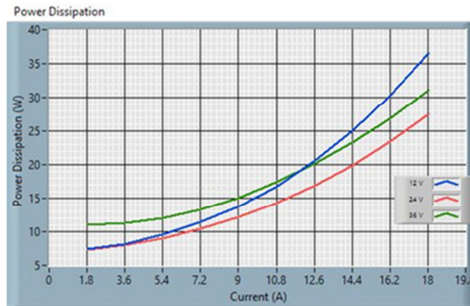
Fig. 9: ICH0518V1PC Power Dissipation
