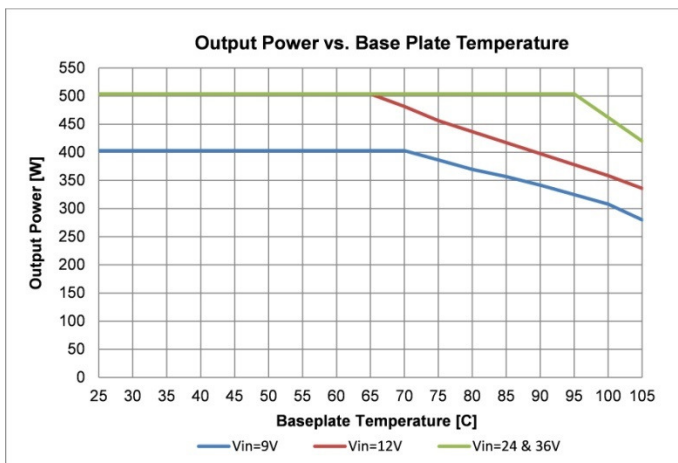
Fig. 14: ICH0518V1PC Derating Curve (P out )
