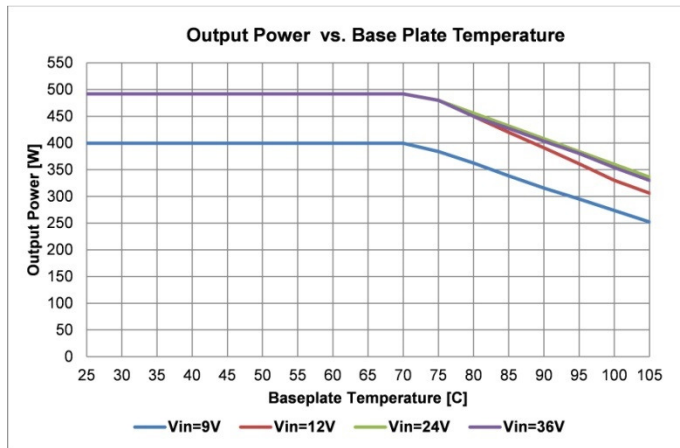
Fig. 10: ICH0141V1PC Derating Curve (P out )
