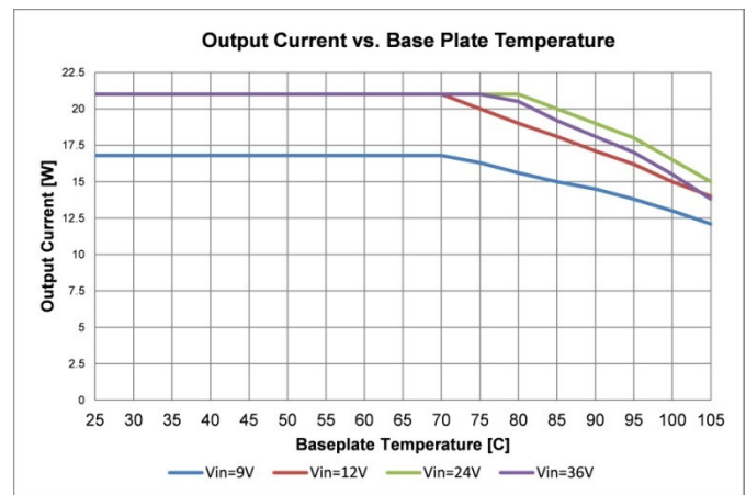
Fig. 13: ICH0421V1PC Derating Curve (I out )
