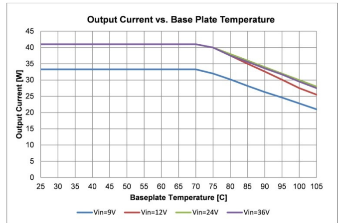
Fig. 11: ICH0141V1PC Derating Curve (I out )
