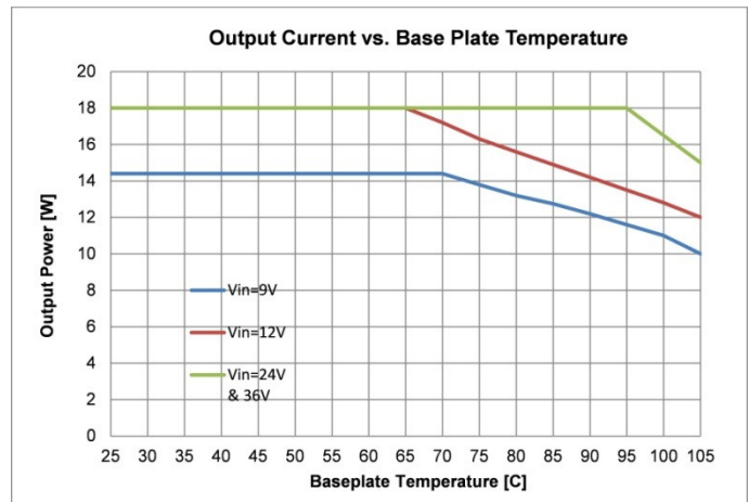
Fig. 15: ICH0518V1PC Derating Curve (I out )
