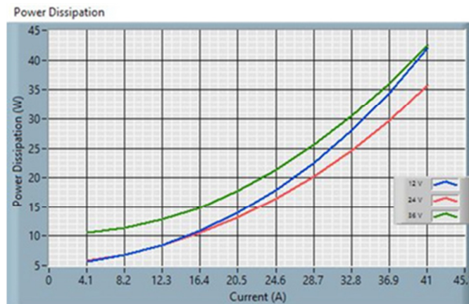
Fig. 5: ICH0141V1PC Power Dissipation
