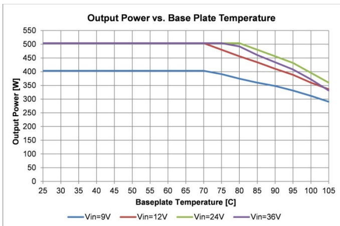
Fig. 12: ICH0421V1PC Derating Curve (P out )
