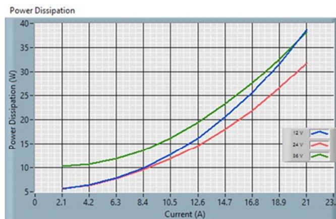
Fig. 7: ICH0421V1PC Power Dissipation
