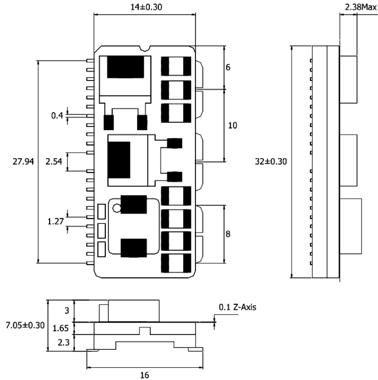
Figure 58. Mechanical Drawing
