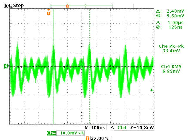
Figure 50. Input Voltage Noise with Interleave
