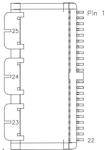
Figure 59. Pinout Diagram (Bottom View)
