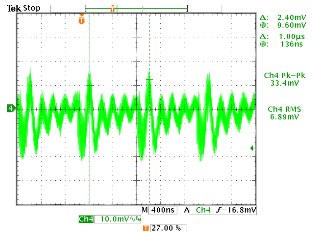
Figure 50. Input Voltage Noise with Interleave
