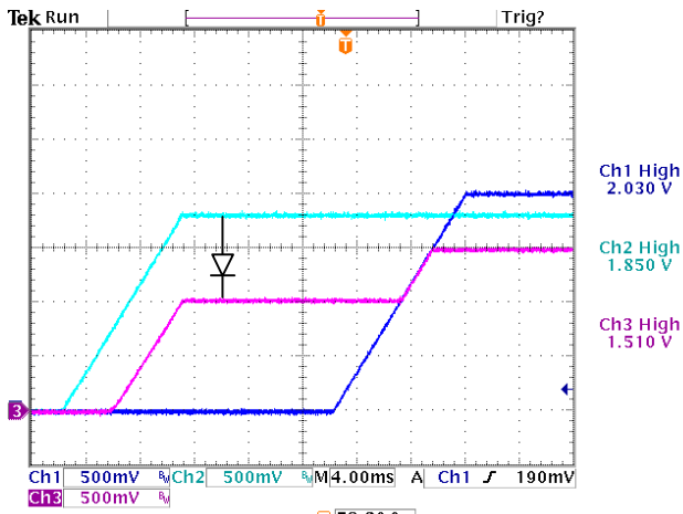
Figure 15. Turn On into Prebiased Load. Same as Figure 14, with a Diode Between V2 and V3. V3 is Prebiased by V2 via the Diode. Vin=12V, Ch1 – V1, Ch2 – V2, Ch3 – V3
