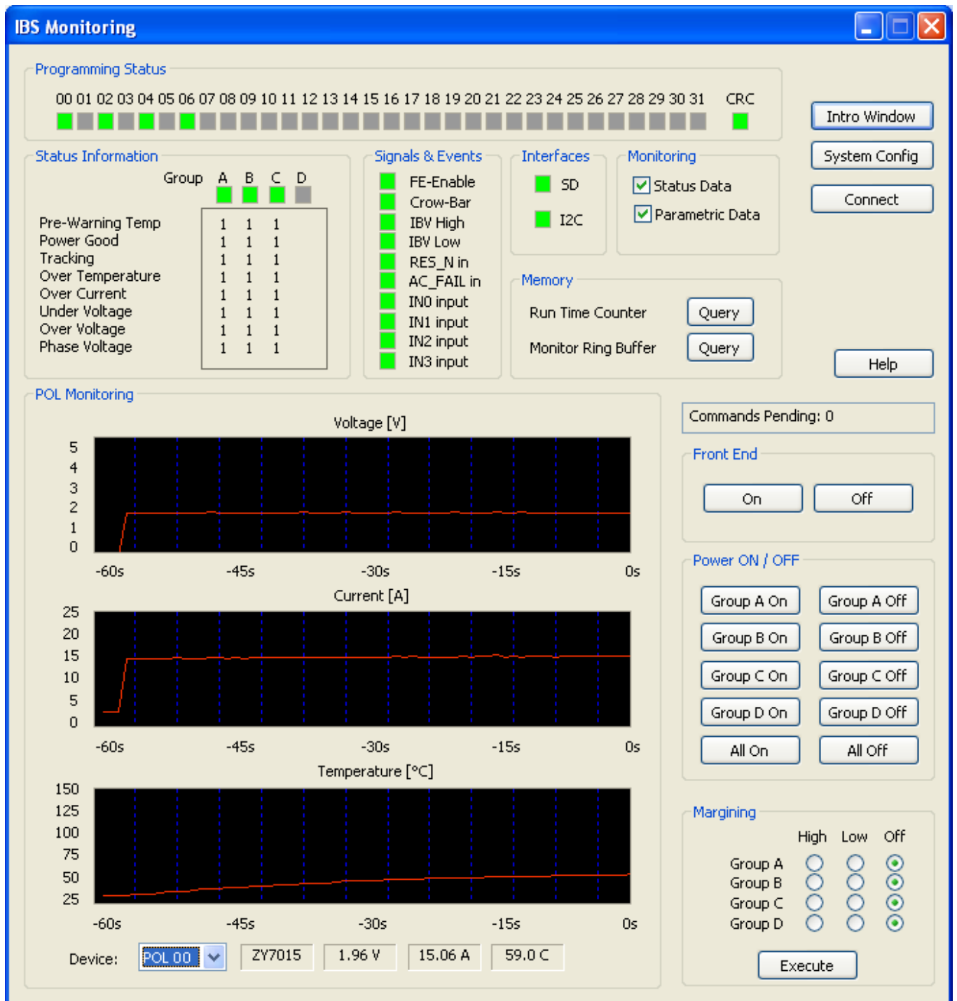
Figure 57. IBS Monitoring Window
