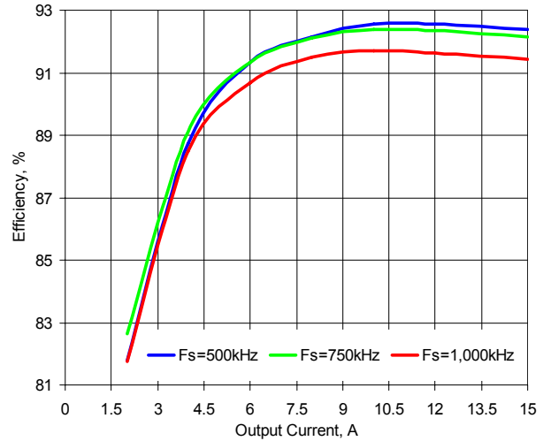
Figure 9. Efficiency vs. Load. Vin=12V, Vout=5V
