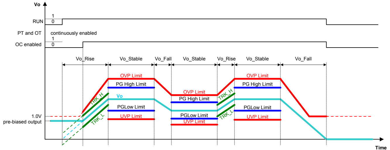
Figure 42. Protections Enable Conditions
