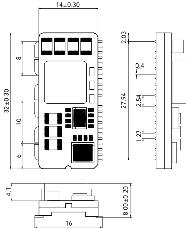
Figure 58. Mechanical Drawing
