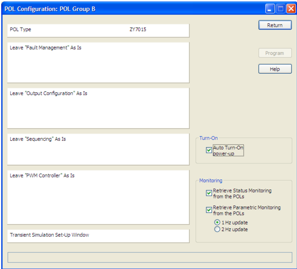
Figure 56. POL Group Configuration Window
