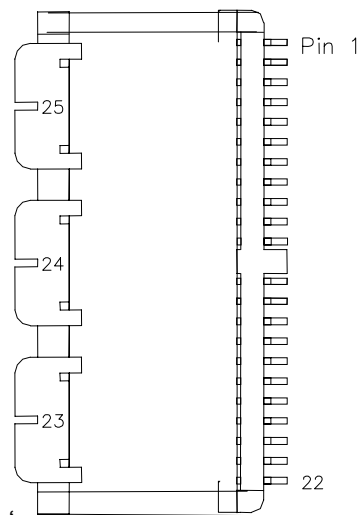
Figure 58. Mechanical Drawing
