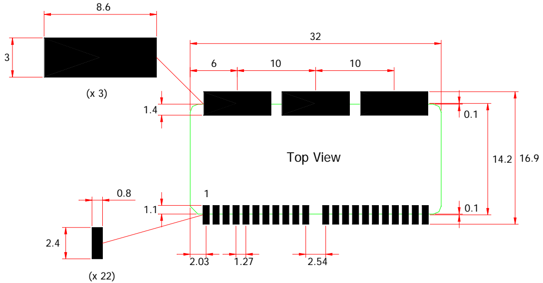
Figure 60. Recommended PCB Pad Sizes
