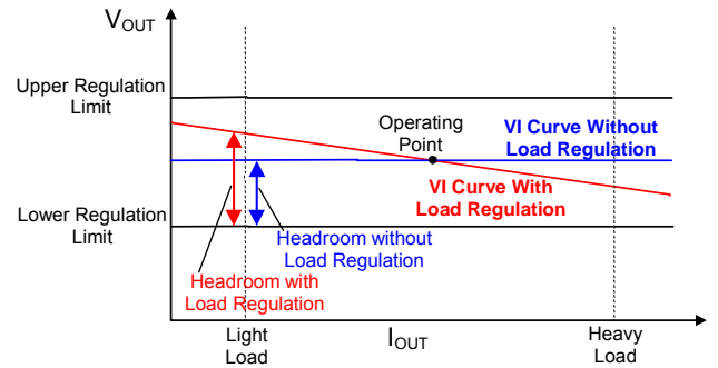
Figure 29. Optimal Voltage Positioning Concept
