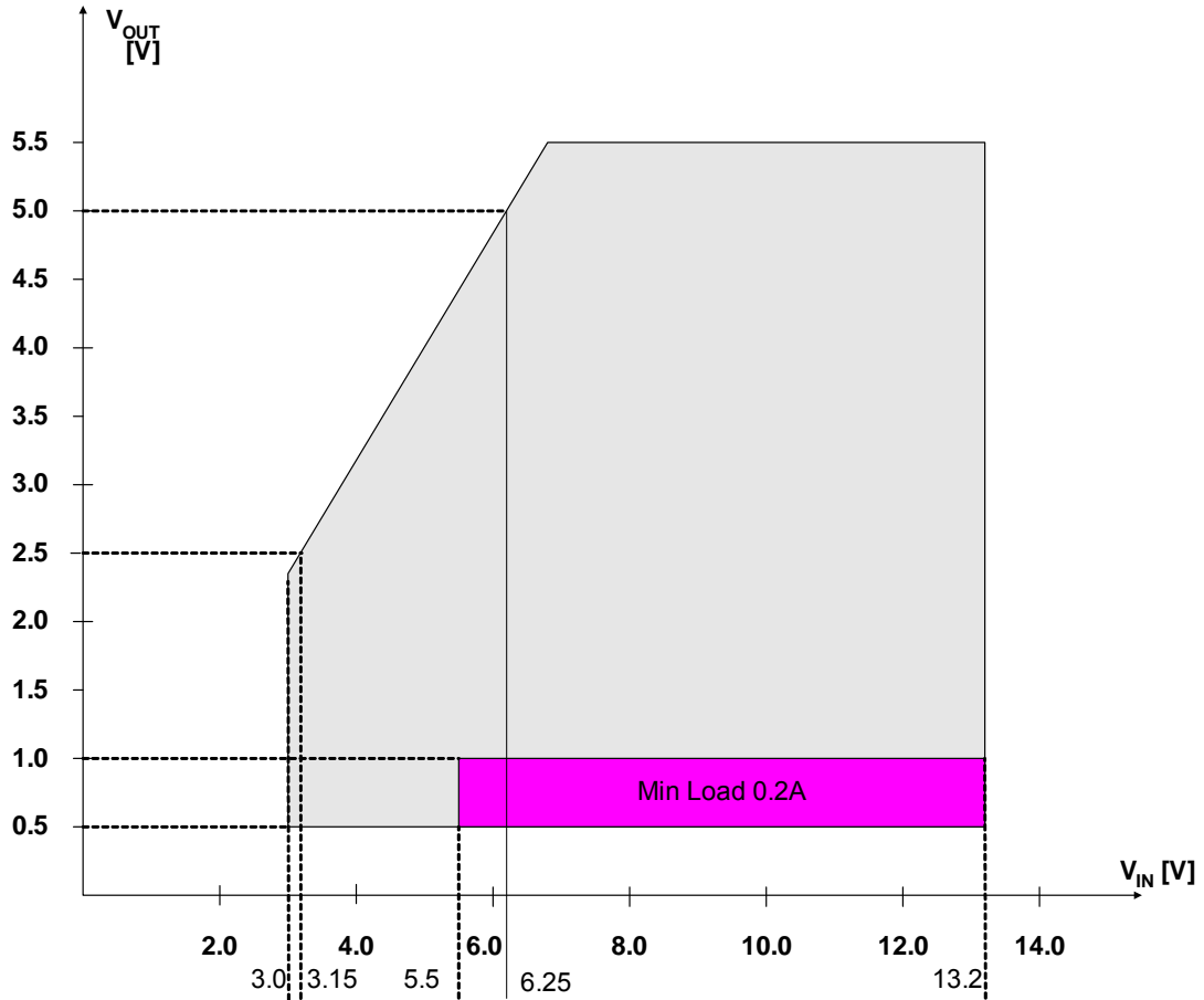
Figure 1. Output Voltage as a Function of Input Voltage and Output Current
