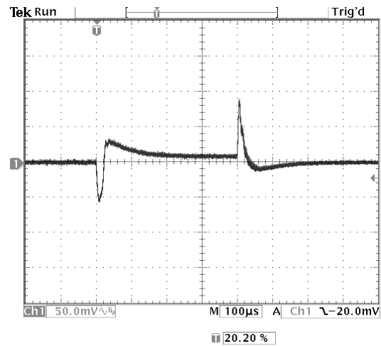
Figure 21. Vin=5V, Vout=1V, BW~40kHz
