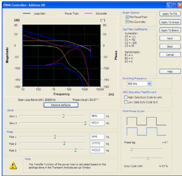
Figure 47. PWM Controller Window
