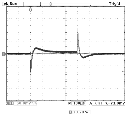
Figure 18. Vin=12V, Vout=5V, BW~40kHz.
