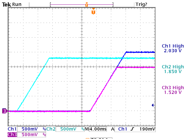
Figure 14. Turn On with Sequencing and Tracking. Rising Slew Rate Programmed at 0.2V/ms, V1 and V3 delays are programmed at 20ms. Vin=12V, Ch1 – V1, Ch2 – V2, Ch3 – V3
