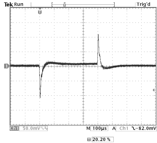
Figure 20. Vin=5V, Vout=2.5V, BW~40kHz
