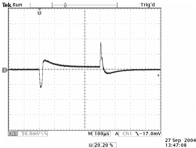
Figure 19. Vin=12V, Vout=1V, BW~40kHz
