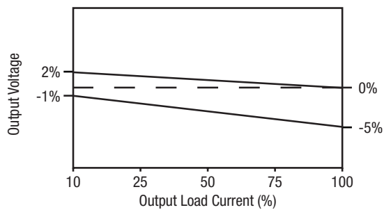
DUAL 0512, SINGLE 1209, 1509
