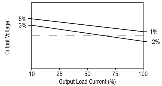
DUAL 1205, 0505, 1505, 2405
