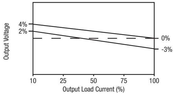
SINGLE 1205, 1505, 2405, 0515
