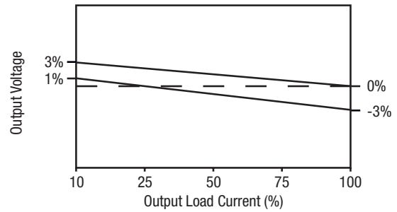
DUAL 1512, SINGLE 1212, 1512, 2412
