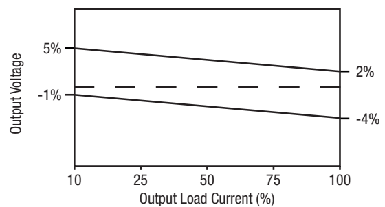
DUAL 1212, 1215, 2415, SINGLE 0509, 0512, 1215, 2409
