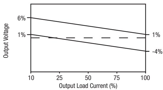
DUAL 0509, 0503, SINGLE 0503, 0505
