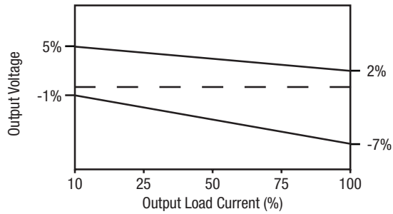
DUAL 0515, SINGLE 1515, 2415
