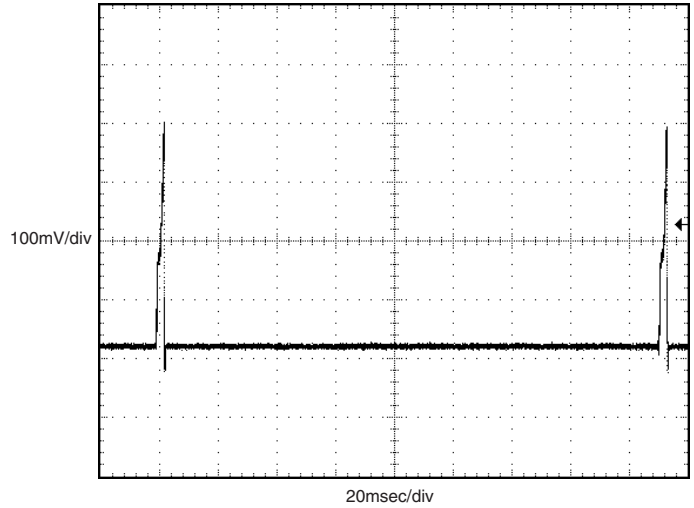
Output Hiccup (LSM-5/10-D12 Shorted VOUT, VIN = 12V)
