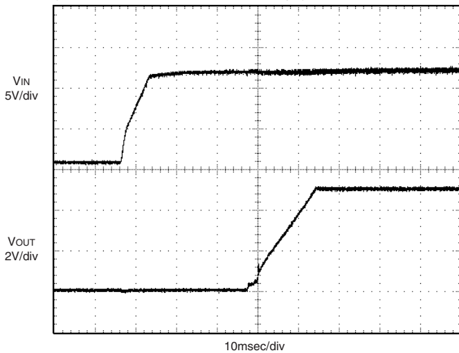
Start-Up from VIN (VIN = 12V, IOUT = 5V/10A, COUT = 22μF)
