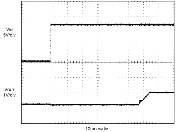
Start-Up from ON/OFF (VIN = 12V, IOUT = 0.8V/10A, COUT = 22μF)
