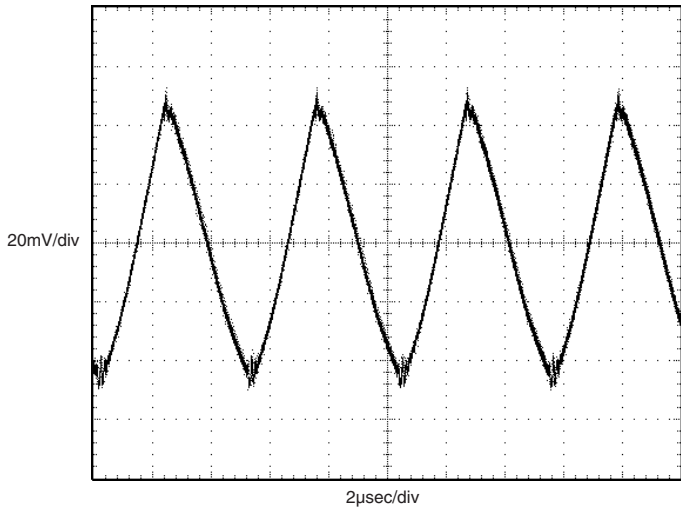
Output Ripple and Noise (VIN = 12V, VOUT = 5V/10A, COUT = 22 \mu F)
