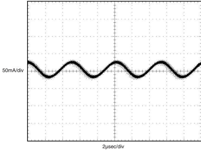
Input Reflected Ripple Current (Input Filter = 220 \mu F/12 \mu H/33 \mu F, VIN = 12V, IOUT = 5V/10A)
