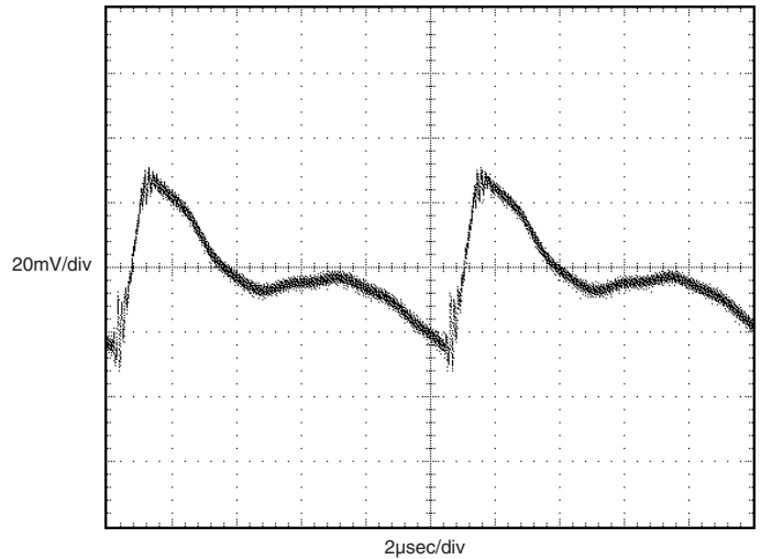
Output Ripple and Noise (VIN = 12V, VOUT = 0.8V/10A, COUT = 22 \mu F)
