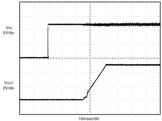
Start-Up from ON/OFF (VIN = 12V, IOUT = 5V/10A, COUT = 22μF)
