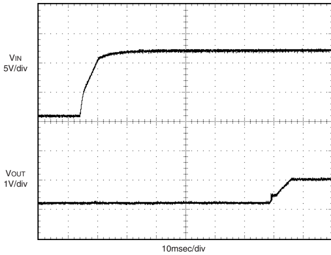
Start-Up from VIN (VIN = 12V, IOUT = 0.8V/10A, COUT = 22μF)
