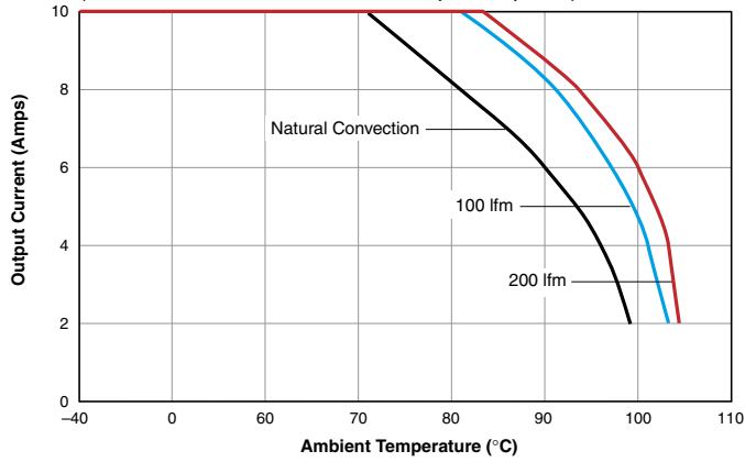
LSN-1.8/10-D3 & LSN-2/10-D3
