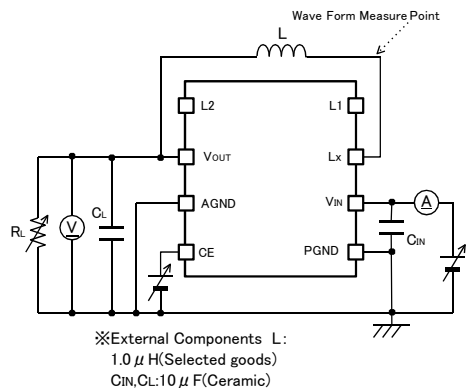
< Circuit No.① >
