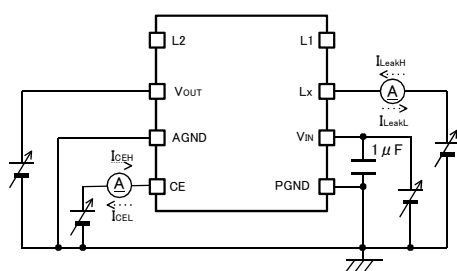
< Circuit No.⑦ >
