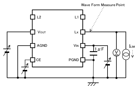
< Circuit No.⑥ >
