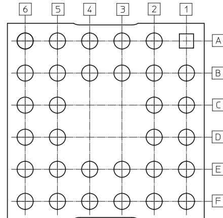
Pin layout, bottom view.
