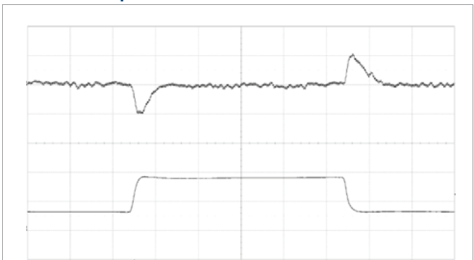
Output voltage response to load current step change (3–9 A) at V_I = 12\text{ V} , C_O = 3 \times 100\ \mu\text{F} + 270\ \mu\text{F}/10\text{m}\Omega . Default compensation settings. Scale: 50 mV/div, 5 A/div, 50 \mu\text{s} /div.
