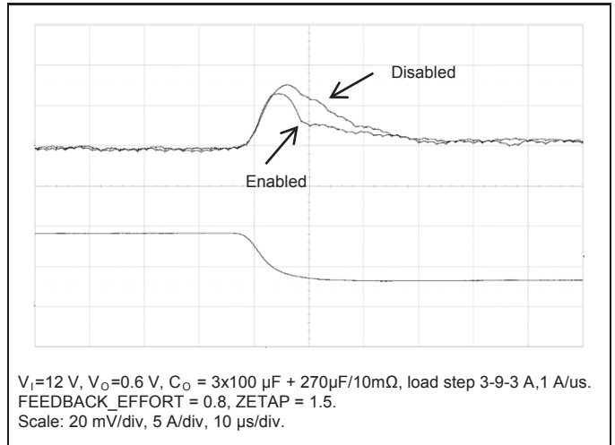
Load release response at enabled/disabled Negative Duty Cycle at low output voltage.
