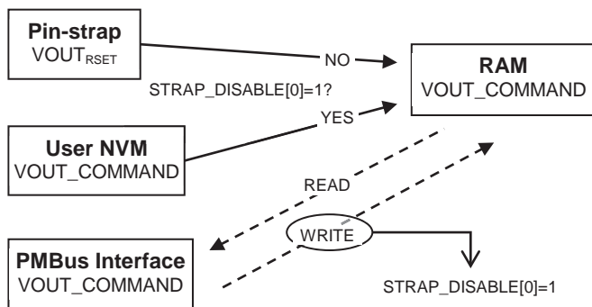
Loading of nominal output voltage level
