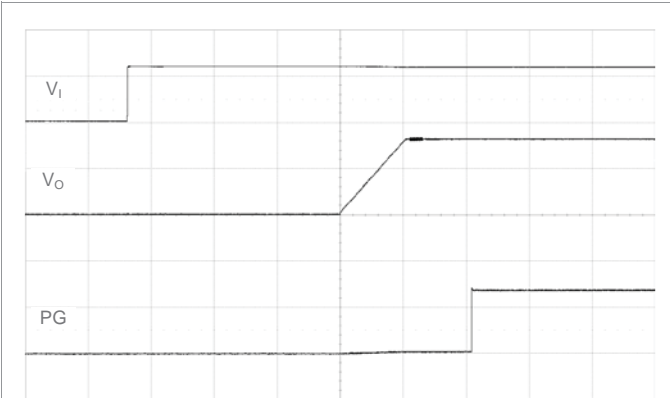
Start-up enabled by applying V_I . \text{TON\_DELAY} = \text{TON\_RISE} = 10\text{ ms} (default). V_I = 12\text{ V} , I_O = \text{max } I_O , PG pulled up to V_O . Scale: 10 or 1 V/div, 10 ms/div.
