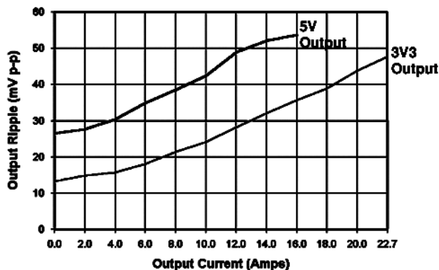
OUTPUT RIPPLE VS. LOAD
