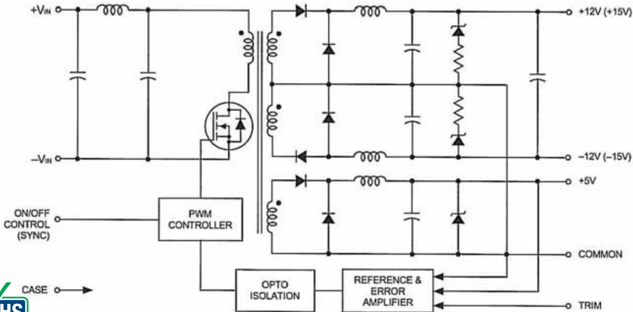
Figure 1. Simplified Schematic
