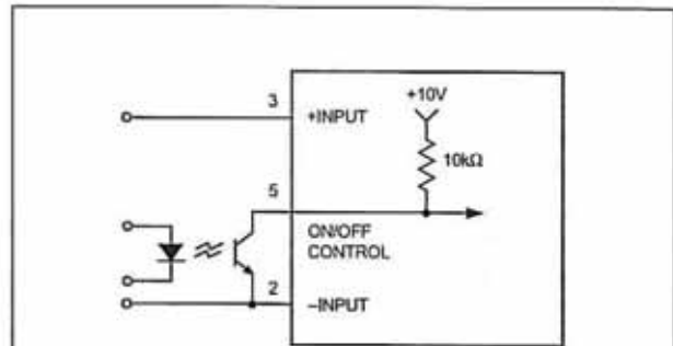
Figure 6. Driving the On/Off Control Pin
