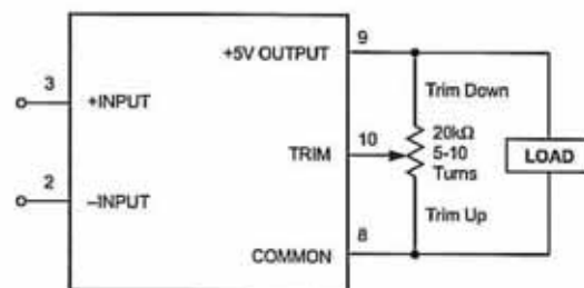
Figure 7. Trim Connections Using a Trimpot
