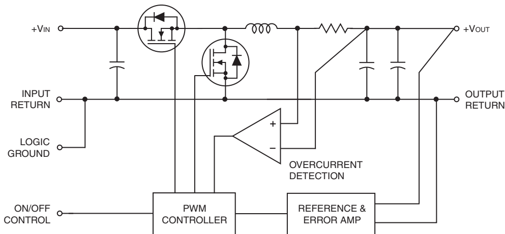
Figure 1. Simplified Schematic
