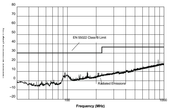
EN 55022 Class B, 10 Meters Converter Output = 3.3Vdc @ 6.4A
