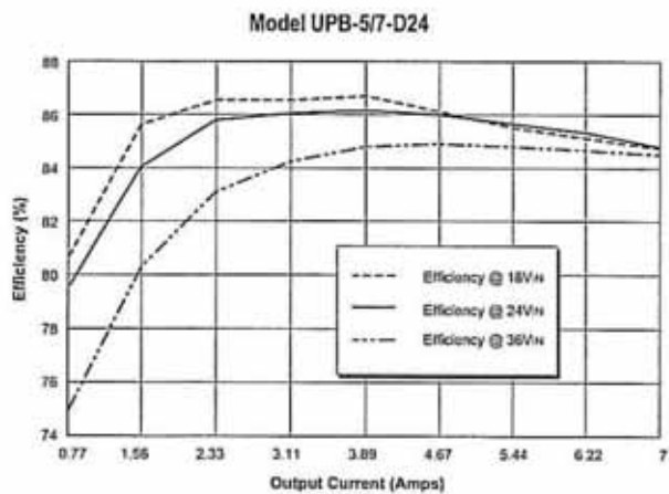
Figure 4c. Efficiency vs. Output Current and Input Voltage
