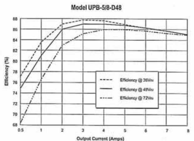
Figure 5c. Efficiency vs. Output Current and Input Voltage
