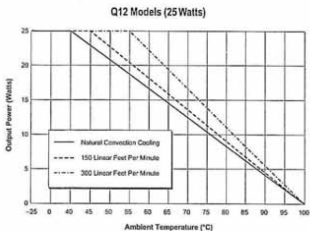
Figure 2a. Temperature Derating Without Heat Sink
