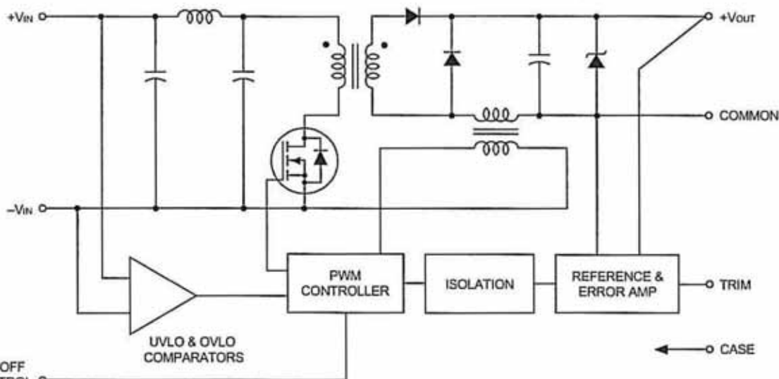
Figure 1. Simplified Schematic
