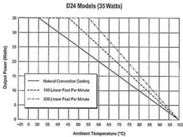
Figure 4a. Temperature Derating Without Heat Sink
