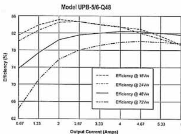
Figure 3c. Efficiency vs. Output Current and Input Voltage
