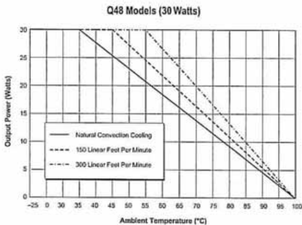
Figure 3a. Temperature Derating Without Heat Sink
