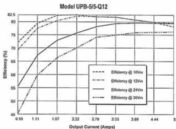
Figure 2c. Efficiency vs. Output Current and Input Voltage
