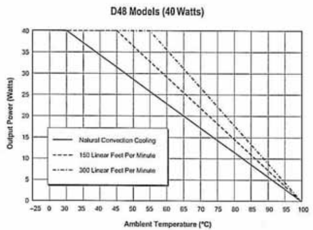
Figure 5a. Temperature Derating Without Heat Sink
