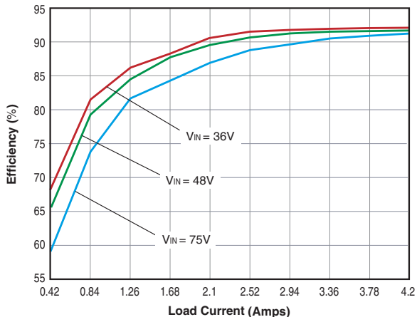
USQ-24/4.2-D48 Efficiency vs. Line Voltage/Load Current @ 25°C
