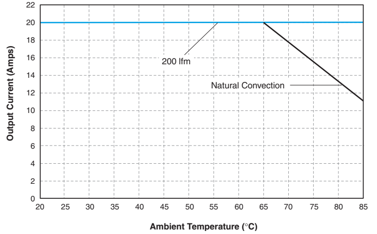
USQ-1.2/20-D48: Maximum Output Current vs. Ambient Temperature (Transverse air flow, pin 1 to pin 3; V_{IN} = 48V , no heat sink.)
