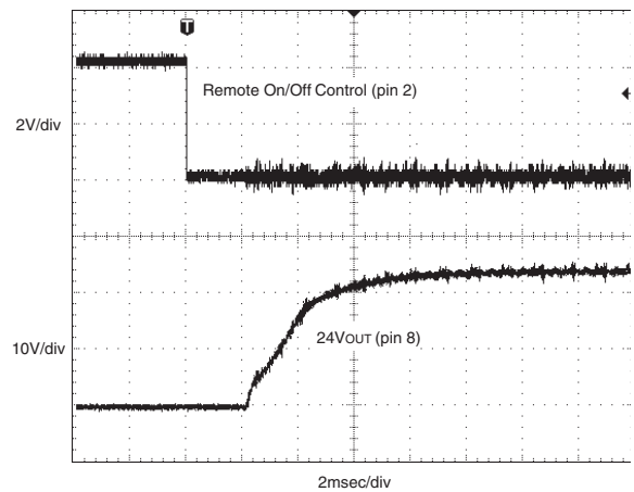
Start-Up from Remote On/Off Control (V IN = 48V, I OUT = 4.2A, C OUT = 10µF tantalum || 1µF ceramic.)
