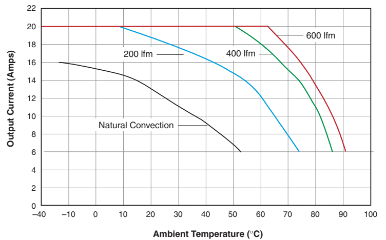
USQ-5/20-D48: Maximum Output Current vs. Ambient Temperature (Longitudinal air flow, pin 1 to pin 4; VIN = 48V, no heat sink.)
