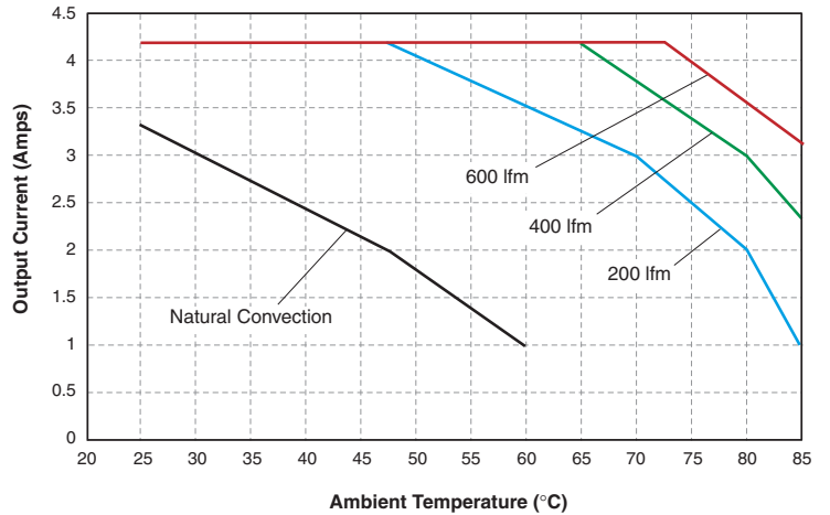
USQ-24/4.2-D24: Maximum Output Current vs. Ambient Temperature (Transverse air flow, pin 1 to pin 3; V IN = 24V, no heat sink.)
