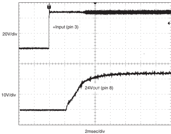
Start-Up from V IN (V IN = 48V, I OUT = 4.2A, C OUT = 10µF tantalum || 1µF ceramic.)
