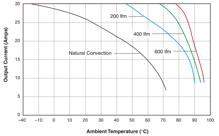
USQ-1.2/30-D48: Output Current vs. Ambient Temperature (Transverse air flow, pin 1 to pin 3; V IN = 48V, no heat sink.)
