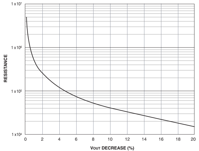
Figure 13. USQ-1.5 to USQ-15 Trim-Down Resistance vs. % Decrease Vout
