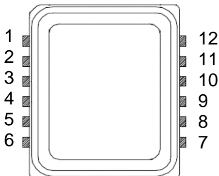
Figure 8: Component pinout
