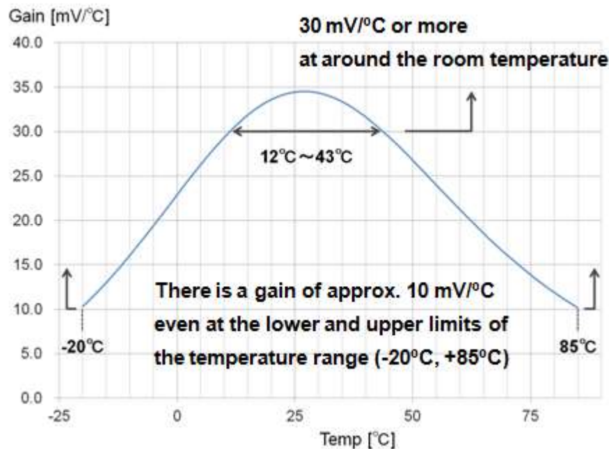
Figure 4. Voltage gain
