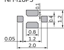
NFM18PS
