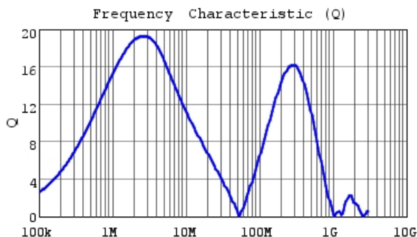
1229AS-H-6R8M Q
