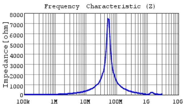
1229AS-H-6R8M |Z|
