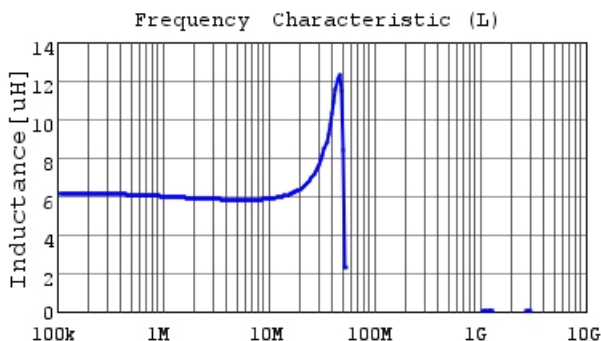
1229AS-H-6R8M L
