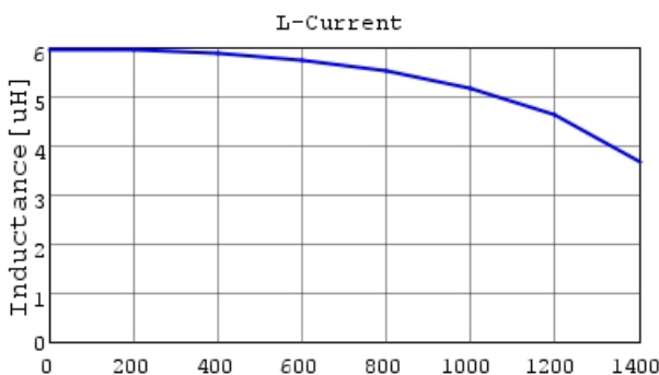
1229AS-H-6R8M L-Current 20degC
